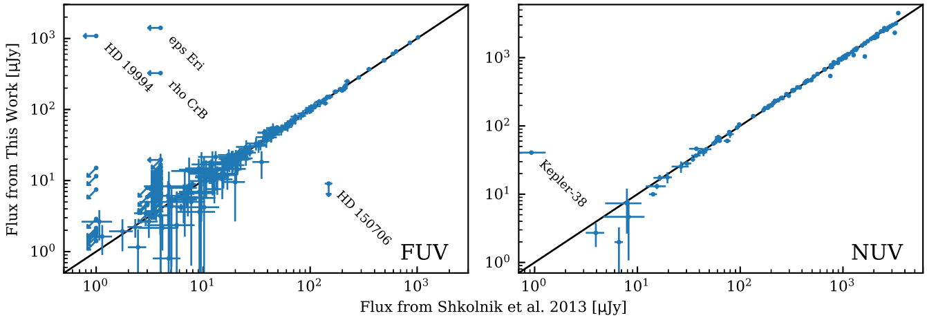
Figure 19. Comparison of GALEX fluxes retrieved by this work vs. Shkolnik (2013). Agreement is good, with most scatter likely due to differences in choice of synthetic aperture, sigma clipping, and method of extracting limits. In a few cases, the GALEX source catalog contained duplicate NUV-only and FUV-only detections of the same source, resulting in false negatives if these duplications were not found.
