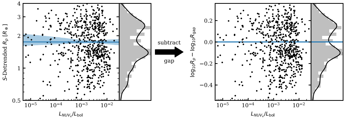
Figure 7. Planetary radius gap in the R_p - L_{\text{NUV}_e}/L_{\text{bol}} (fractional \text{NUV}_e luminosity of the star) plane after removing the dependence from the R_p - S fit shown in Figure 3. The blue line and translucent area are the best fit to the gap and bootstrapped 1\sigma uncertainty. In the right panel, the best fit has been subtracted in log space, aligning the gap to the histogram. The slope of the radius gap is consistent with zero, implying that differences in the \text{NUV}_e portion of a planet’s installation are not associated with detectable changes in the radius gap.
