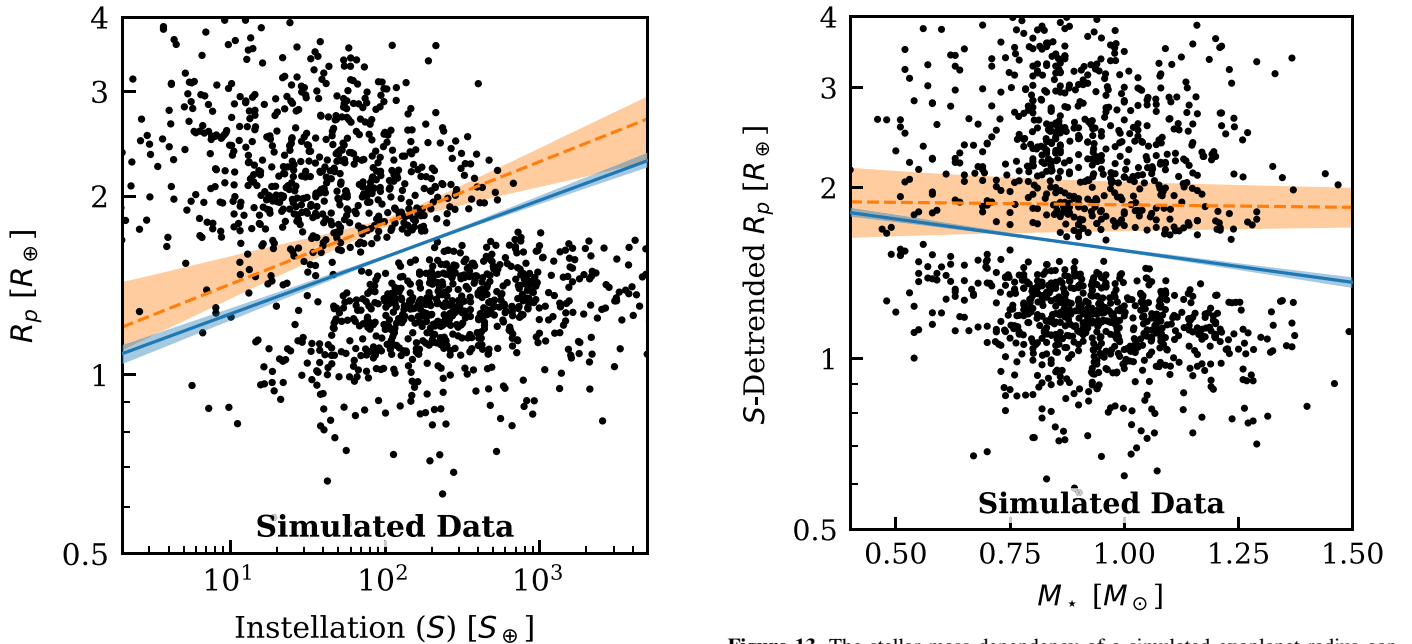
Figure 12. The instellation dependency of a simulated radius gap generated by XUV evaporation. The simulated population in this figure can be directly compared to the real planetary population in the left panel of Figure 3. The radius gap has a slope of 0.096^{+0.009}_{-0.008} (blue line) in agreement with the slope of the radius gap in the actual planet population (orange line) of 0.10^{+0.02}_{-0.04} . See text for discussion of the offset between the simulated and actual radius gaps.
