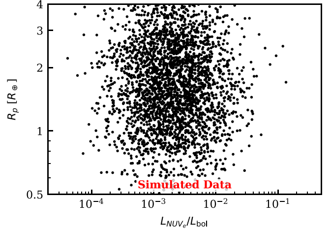
Figure 24. The simulated planet population plotted in the R_p - L_{\text{NUV}_e}/L_{\text{bol}} plane. The gap has been obscured due to the scatter from the large range of possible \text{NUV}_e irradiation for planets with similar L_{\text{NUV}_e}/L_{\text{bol}} , which drives the radius of the gap in this idealized sample.
