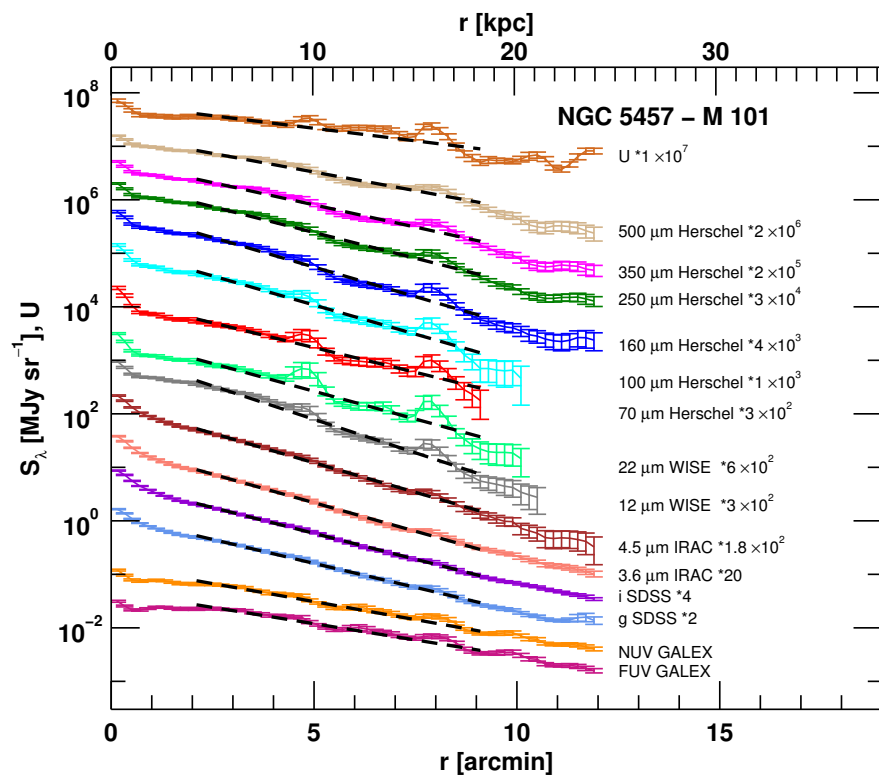
Fig. 2. Multi-wavelength surface brightness profiles for the galaxy NGC 5457 (M 101), shown up to r_{25} . The profiles have been shifted for displaying purposes and the corresponding offsets are quoted next to each profile. The profiles are arranged in order of decreasing wavelength, from top to bottom. At the top, the interstellar radiation field intensity U , is shown, in dimensional units. The black dashed lines are exponential fits performed avoiding the central part of galaxies up to the maximum extension of the 70 \mu\text{m} profile (shown in red).
