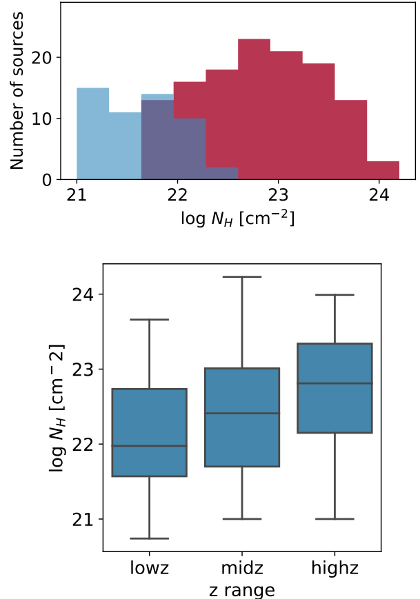
Fig. 3. Upper panel: distribution of best-fit N_{\text{H}} values obtained for all the 180 sources at z > 0.4 . The histogram in red shows the N_{\text{H}} distribution of absorption detected sources, while the blue histogram shows that of the upper limits. We note the limited but uniform sensitivity of our spectra to N_{\text{H}} due to the rest-frame bandpass (see text). Lower panel: box-and-whisker plots of N_{\text{H}} measurements for the lowz, midz and highz groups. Following the normal convention, the box represents the inter quartile range (the middle 50%), the bar in the middle represents the median value, and the whiskers show the range of the minimum and the maximum of the distribution.
