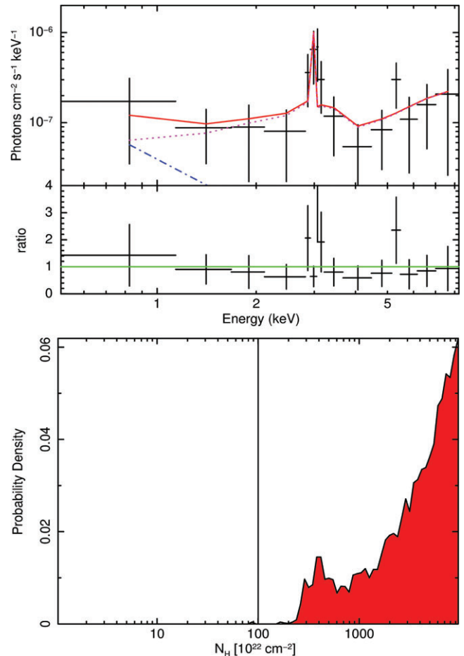
FIGURE 6 Same as Figure 5, for source LID_390.
