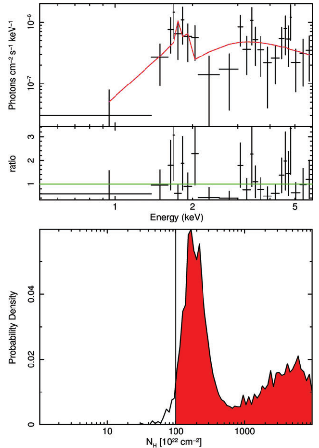
FIGURE 2 (a) Unfolded spectrum and data/model ratio of the CT candidate LID_1002 at z=2.612 . This source required only the BNTorus component. (b) PDF of N_{\text{H}} for the same source.
