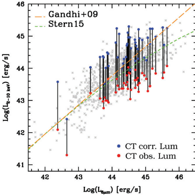
FIGURE 3 Distribution of the AGN mid-IR ( 6\ \mu\text{m} ) luminosity, as derived from SED fitting, after subtracting the host star-formation emission, and the 2–10 keV luminosity, for the \sim 2,000 sources analyzed in Marchesi et al. (2016a) (gray crosses). Red circles show the observed L_X for the CT candidates, while blue circles show the absorption-corrected L_X . The orange (green) curve shows the relation published in Gandhi et al. (2009) (Stern 2015).
