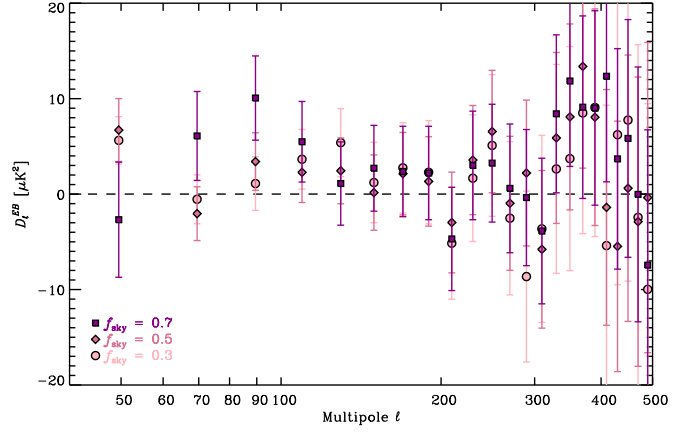
Fig. B.3: Planck HFI 353 GHz \mathcal{D}_\ell^{EB} power spectra (in \mu\text{K}_{\text{CMB}}^2 ) computed on three of the selected LR analysis regions that have f_{\text{sky}} = 0.3 (circles, lightest), f_{\text{sky}} = 0.5 (diamonds, medium), and f_{\text{sky}} = 0.7 (squares, darkest). The uncertainties plotted here are \pm 1\sigma .
