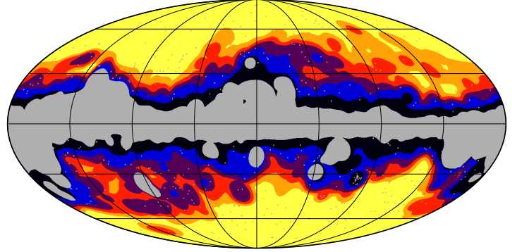
Fig. 1: Masks and complementary selected large regions that retain fractional coverage of the sky f_{\text{sky}} from 0.8 to 0.3 (see details in Sect. 3.3.1). The gray is the CO mask, whose complement is a selected region with f_{\text{sky}} = 0.8 . In increments of f_{\text{sky}} = 0.1 , the retained regions can be identified by the colours yellow (0.3) to black (0.8), inclusively. Also shown is the (unapodized) point source mask used.
