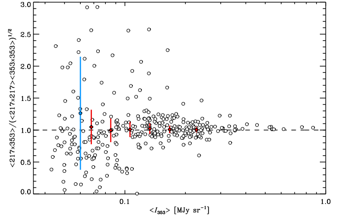
Fig. E.1: Ratio of the 217 \times 353 \mathcal{D}_\ell^{BB} cross-spectrum amplitude with respect to the geometrical mean between the 217 GHz and 353 GHz \mathcal{D}_\ell^{BB} auto-spectrum amplitudes, as a function of \langle I_{353} \rangle for the region on which the spectra are computed. These ratios are presented for the 352 patches of Sect. 5 (black circles, with error bars not presented for the sake of clarity), for the six LR regions of Sect. 4 (red diamonds) and for the M_{B2} region of Sect. 6 (blue diamond).
