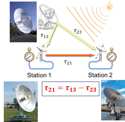
Fig. 1 NHS scheme and the three antennas involved in the project: above Kashima, on the left MLB1 installed at the Medicina Observatory and on the right MLB2 located in Koganei.
