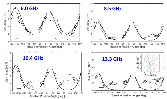
Fig. 3 Model of the frequency dependent source size for 1928+738.
