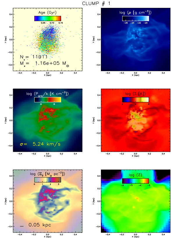
Figure 10. Main properties of clump 1 of Fig. 9 and slice maps of various properties of the gas, each one centred on the centre of mass of the clump. Top left-hand panel: scatter plot of the stars, colour-coded with their age. Top right-hand panel: gas density map. Middle left-hand panel: pressure map. Middle right-hand panel: temperature map. Bottom left-hand panel: gas surface density. Bottom right-hand panel: metallicity map. The density, temperature, and metallicity maps are computed as mass-weighted averages along the line of sight. For the gravitational pressure and surface density we show column density maps, in which the quantities are summed along the line of sight.
