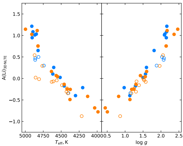
Fig. 12. Lithium abundances in respect of the effective temperature and surface gravity values for stars in metal-rich (blue symbols) and metal-poor (orange symbols) populations. The upper values of Li abundances are plotted by empty circles.
