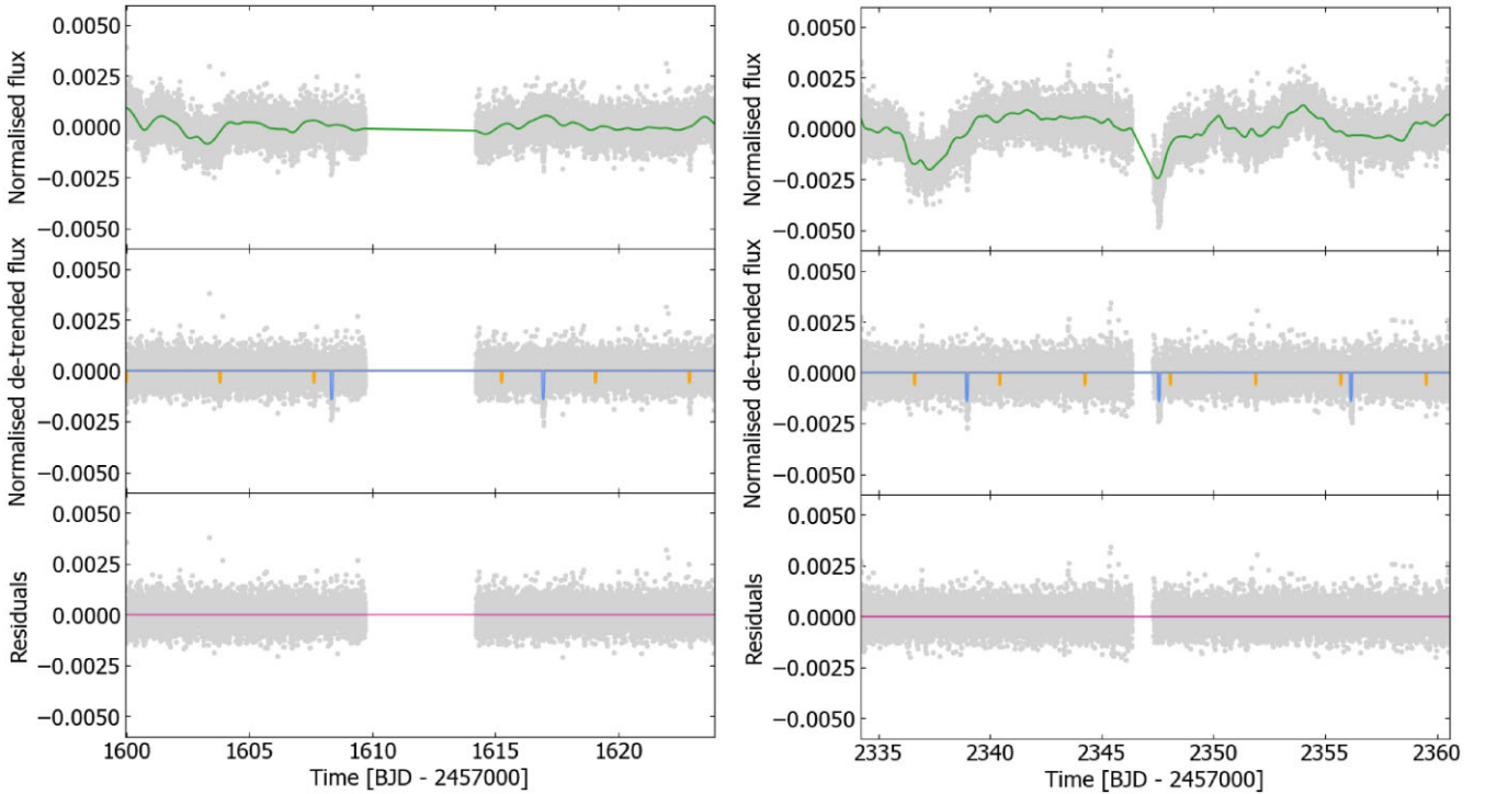
Figure 2. Top left-hand panel: TESS PDC-SAP light curve from Sector 11 with the GP model plotted in green. Middle left-hand panel: TESS PDC-SAP light-curve data minus the GP model, with transits plotted for TOI-836 c (blue line) and TOI-836 b (orange line). Bottom left-hand panel: Residuals between the best-fitting model and the TESS data points. Top right-hand panel: TESS PDC-SAP light curve from Sector 38 with the GP model plotted in green. Middle right-hand panel: TESS PDC-SAP light-curve data minus the GP model, with transits plotted for TOI-836 c (blue line) and TOI-836 b (orange line). Bottom right-hand panel: Residuals between the best-fitting model and the TESS data points.
