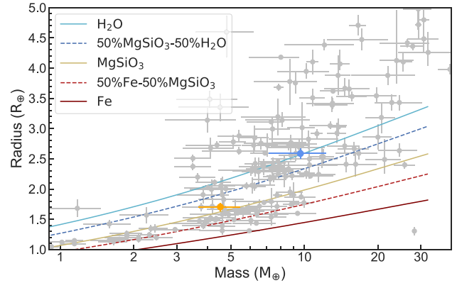
Figure 13. Mass-radius diagram plotted for TOI-836 b in orange and TOI-836 c with exoplanets from the TEPCAT catalogue (Southworth 2011) in grey and composition models from Zeng, Sasselov & Jacobsen (2016).
