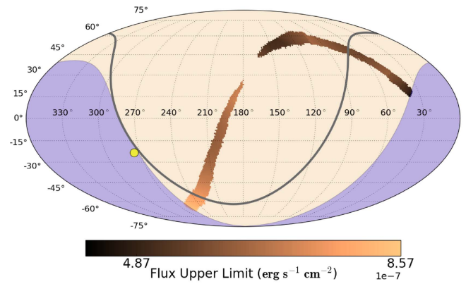
Figure 5. The area within the GW151226 LIGO localization contour is shaded to indicate the GBM 10–1000 keV flux upper bounds during the the T_{\text{seeded}} interval: -30 < t_{\text{GW}} < +30 s. The purple shaded region indicates where the sky was occulted by the Earth for Fermi . The Galactic plane is the gray curve, and the Sun is indicated by the yellow disk.
