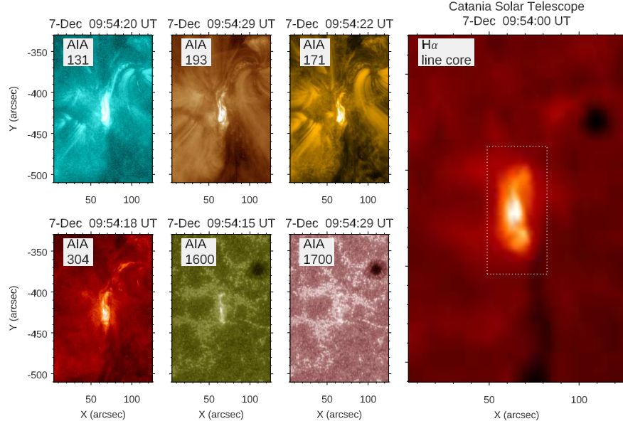
Figure 5. Simultaneous multi-wavelength observations during the peak of the SOL2020-12-07T09:55 flare. Left panels: Maps derived from SDO/AIA observations corresponding to filters with decreasing temperature formation, from EUV 131 Å down to UV 1700 Å. Right panel: H \alpha observation acquired with the Catania Solar Telescope. The dashed box in the H \alpha map indicates the subFOV used for computing the light curve shown in Figure 6 and for studying the sequence of IRIS observations shown in Figure 8.
