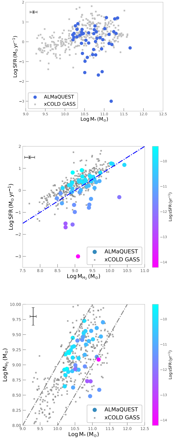
Figure 3. Top panel: Distribution of the ALMaQUEST galaxies (blue symbols) in the global SFR and M_{*} plane. For comparison, the xCOLD GASS sample is shown as the grey squares and only galaxies with CO detections are shown for clarity. Middle panel: distribution of the ALMaQUEST galaxies in the global Schmidt-Kennicutt relation (SFR vs. M_{*} ) color-coded by sSFR. The blue dot-dashed line corresponds to the \text{SFE} = 10^{-9} \text{ yr}^{-1} line, not the best-fit to the data. Bottom panel: Relation between the global M_{\text{H}_2} and M_{*} (global molecular gas main sequence) of the ALMaQUEST sample color-coded by sSFR. The two grey dot-dashed lines, from left to right, show a gas-to-stellar ratio of 0.1 and 0.01, respectively. For the three panels, all of the ALMaQUEST quantities (i.e., SFR, M_{*} , M_{\text{H}_2} ) are computed within 1.5 R_e . The black error bars shown in the upper left corners represent the typical uncertainties.
