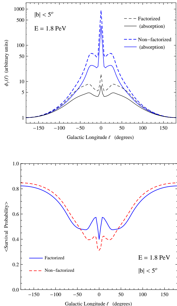
FIG. 14: Top panel: longitude distribution of the gamma ray flux at E = 1.8 PeV, integrated in the latitude range |b| < 5^\circ . The flux is shown for both our models (factorized and non-factorized emissions), including and neglecting the effects of absorption. Bottom panel: average survival probability for gamma rays of energy E = 1.8 PeV, averaged in the latitude interval |b| < 5^\circ , as a function of the Galactic longitude, according to our two models.
