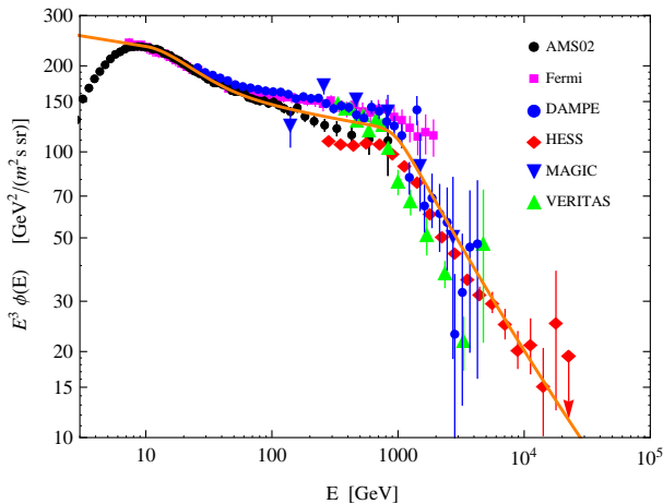
FIG. 3: Flux of electrons plus positrons observed at the Earth. The line is our fit to the spectrum. The data points are from Fermi [37], AMS02 [38], DAMPE [44], HESS [39–41], MAGIC [42] and VERITAS [43].
