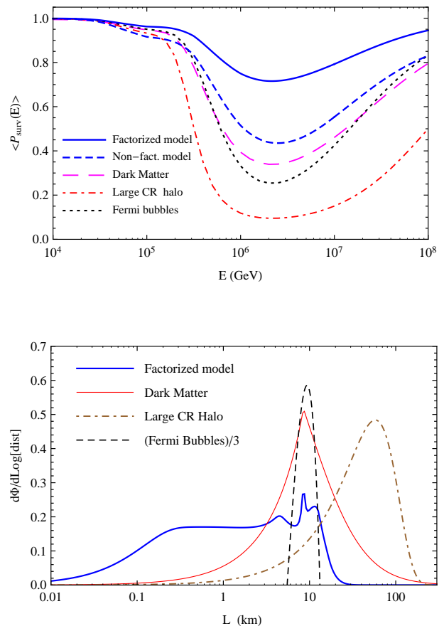
FIG. 18: Top panel: average survival probability of gamma rays (after integration over the entire sky) for different emission models. Bottom panel: distribution of the gamma ray pathlength for the same models. The distributions are calculated after integration over the entire solid angle, neglecting the effects of absorption, and are normalized to unity (or 1/3 for the Fermi bubbles case).
