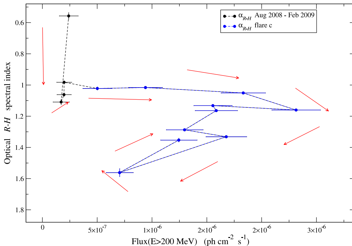
Fig. 23.— Optical R - H spectral index vs. the LAT Flux above 200 MeV. The black points refer to the 2008 August to 2009 February period, and are poorly sampled to be used to investigate the optical/ \gamma -ray connection. The blue points overlap mainly the flare c , in particular the subflare peaking at about MJD 54909 (see fig. 2, panel d). The red arrows shows the chronological sequence.
