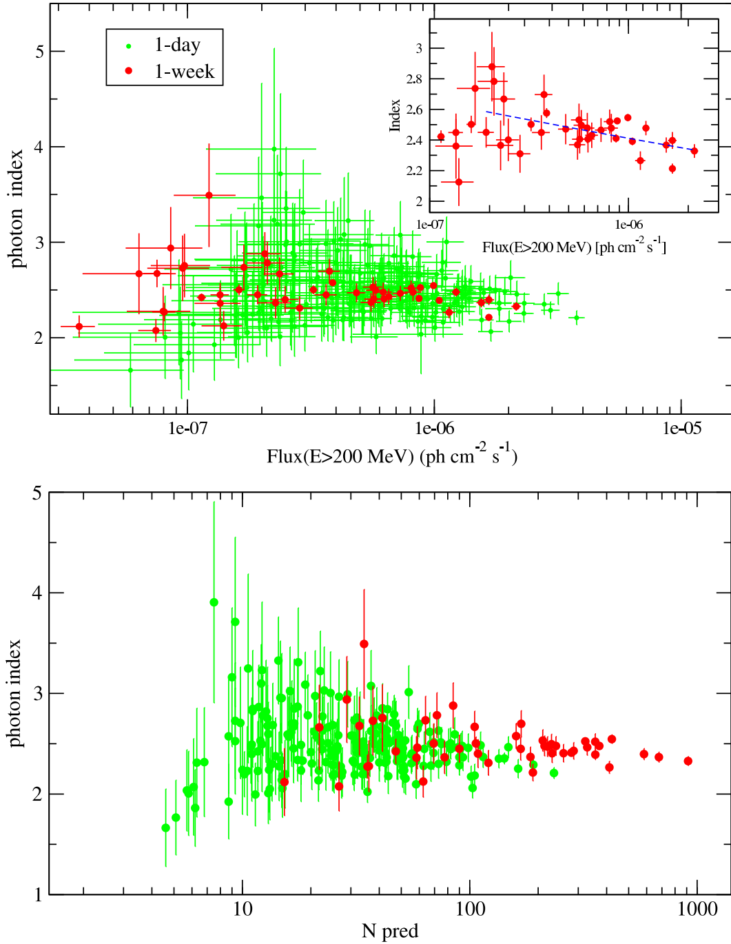
Fig. 5.— Upper Panel: weekly and daily scatter plot of the Flux( E > 200 \text{ MeV} ) vs. the photon index ( \text{TS} > 10 ). The inset shows the same for Flux( E > 200 \text{ MeV} ) > 2 \times 10^{-7} \text{ ph cm}^{-2} \text{ s}^{-1} . Lower Panel: Scatter plot of the number of photons predicted by the best-fit model vs. the photon index, for weekly and daily integration ( \text{TS} > 10 ).
