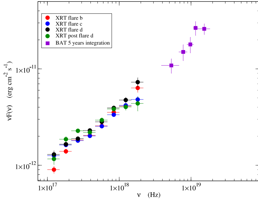
Fig. 9.— XRT SEDs averaged during the flare b , c , d and during the post d flare period. The violet boxes represent the BAT spectrum averaged over 5 years
