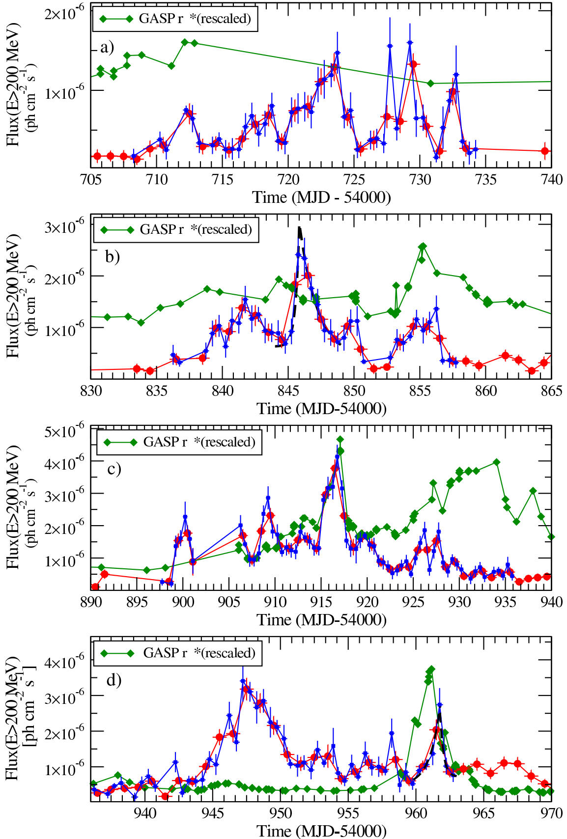
Fig. 2.— from top to bottom, flare a , b , c , and d showing 1-day binning (red points) and 12 hr
