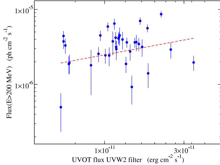
Fig. 14.— Scatter plot of the Fermi -LAT flux ( E > 200 MeV) vs. the UVOT \nu F(\nu) in the UVW2 filter. The red dashed line represents the best-fit power law model. The correlation coefficient of the logarithm of the UV and \gamma -ray fluxes is r = 0.2 with a 95% confidence interval of 0.05 \leq r \leq 0.34 .
