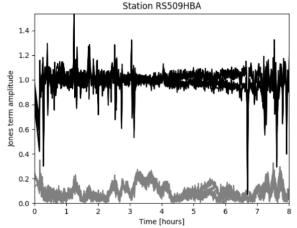
Fig. 3. Amplitude of the diagonal (black) and off-diagonal (gray) terms of the estimated Jones matrices for a remote station using the LOFAR observation synthesized 6'' image as the sky model (self-calibration). If the initial DI calibration and correction by PREFACTOR on the lower resolution TGSS sky model were good enough, the calibration solutions found here would be the unity matrix at all times and frequencies. Therefore, in DDF-PIPELINE-V2, we carry out a few full-Jones DI-only self-calibration steps. This approach seems very efficient in increasing the dynamic range around the brightest radio sources.
