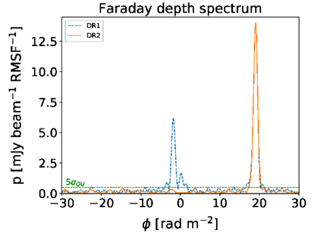
Fig. 7. Faraday depth spectrum, or Faraday dispersion function (FDF), for a radio galaxy in both the DR1 and DR2 datasets, showing the suppression of the instrumental polarization signal. The dashed blue line shows the FDF from the DR1 data with a strong instrumental polarization feature near Faraday depths of \phi \sim 0 \text{rad m}^{-2} , while the solid orange line shows the FDF from the DR2 data in which the instrumental feature is suppressed below the noise level. In both cases, the Faraday depth of the real astrophysical signal is the same.
