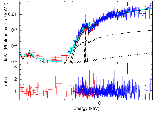
XMM–NuSTAR – UXCLUMPY – February 03–04, 2022
