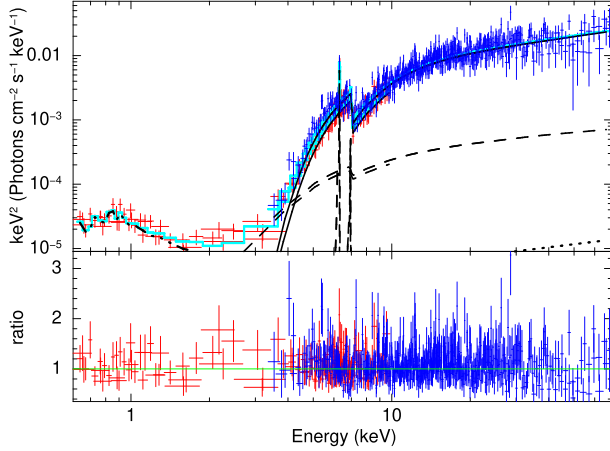
XMM–NuSTAR – borus02 – February 03–04, 2022
