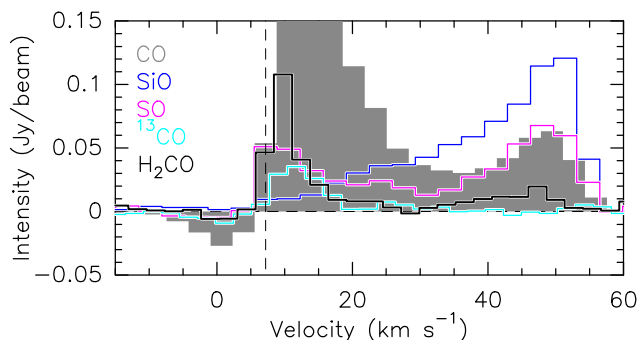
Fig. 6. 12 CO(2–1) (grey), SiO(5–4) (blue), SO(6 5 –5 4 ) (magenta), 13 CO(2–1) (cyan), and p-H 2 CO(3 03 –2 02 ) (black) spectra at the EHV peak (see Fig. 5). The p-H 2 CO(3 03 –2 02 ) spectrum was observed with WideX (see Appendix B) at the spectral resolution of ~2.7 km s -1 ; all other spectra have thus been smoothed to the same spectral resolution. The 12 CO(2–1) data have been convolved to match the angular resolution at 1.4 mm (1'1×0'8).
