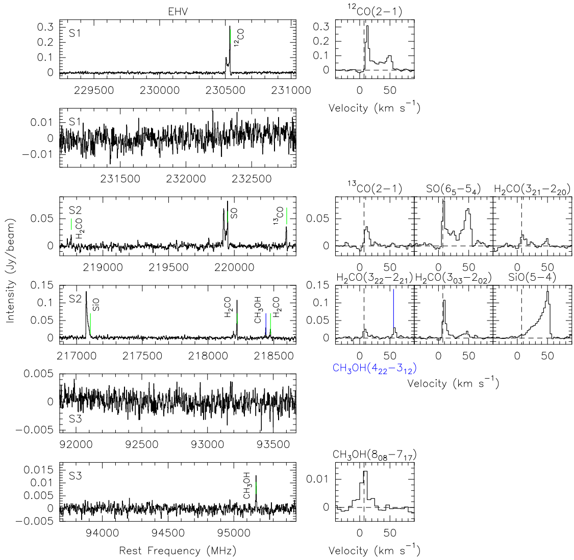
Fig. B.1. Additional lines detected in the WideX spectra at the peak of the EHV gas.
