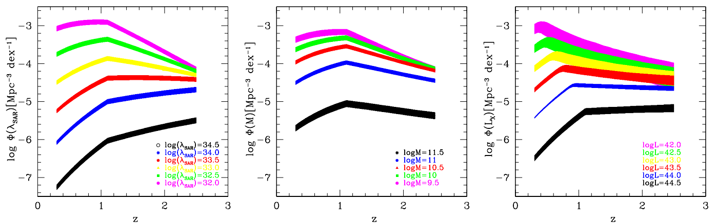
Fig. 5. Left Panel: Redshift evolution of the SARDF space density for different \lambda_{\text{SAR}} , i.e. magenta: \log(\lambda_{\text{SAR}})=32 [ \text{erg}/\text{s}/M_\odot ] ( \sim 1\% Edd); green: \log(\lambda_{\text{SAR}})=32.5 [ \text{erg}/\text{s}/M_\odot ] ( \sim 3\% Edd); yellow: \log(\lambda_{\text{SAR}})=33 [ \text{erg}/\text{s}/M_\odot ] ( \sim 10\% Edd); red: \log(\lambda_{\text{SAR}})=33.5 [ \text{erg}/\text{s}/M_\odot ] ( \sim 30\% Edd); blue: \log(\lambda_{\text{SAR}})=34.0 [ \text{erg}/\text{s}/M_\odot ] ( \sim Edd); and black: \log(\lambda_{\text{SAR}})=34.5 [ \text{erg}/\text{s}/M_\odot ] ( > Edd). Central Panel: Redshift evolution of the HGMF space density for different M_* . Right Panel: Redshift evolution of the XLF space density for different L_X by Miyaji et al. (2015).
