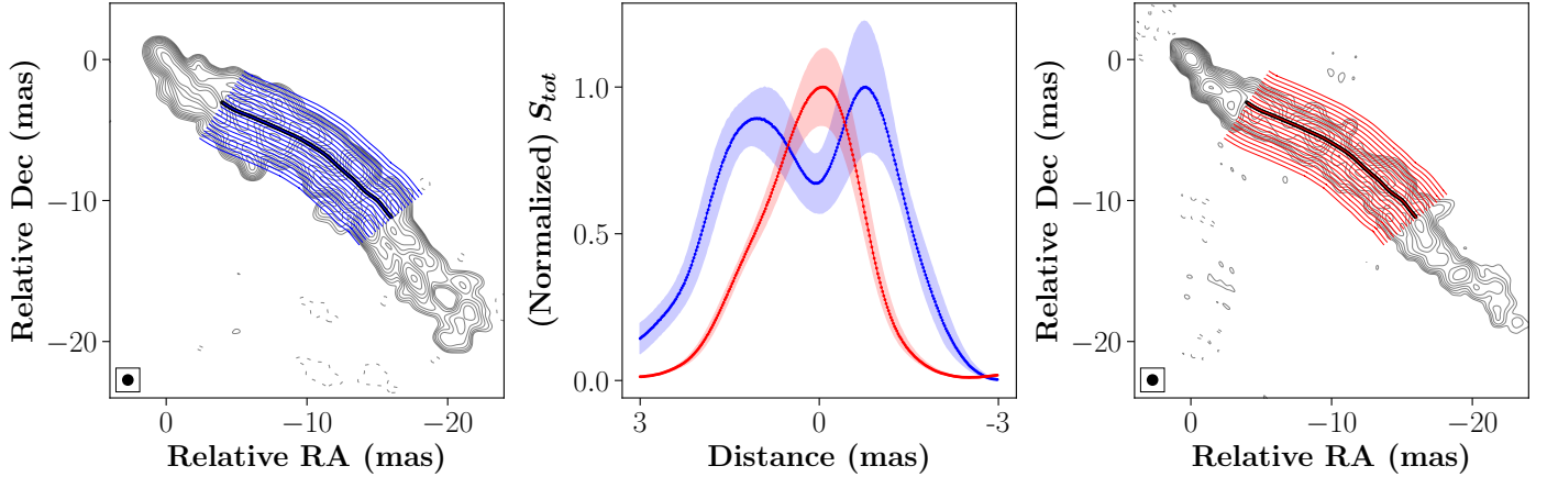
Fig. 5. Jet streamlines (300) used to calculate the integrated flux density along the flow, parallel to the jet axis from MOJAVE (central line in black), overplotted on the 1.6 GHz ( left panel ) and 4.8 GHz ( right panel ) RadioAstron contours maps (both convolved with the MOJAVE beam). The starting point is set at 4 mas from the core, where the spine/sheath structure becomes evident. Central panel : integrated flux density, versus distance from jet axis, calculated along jet streamlines for the 1.6 GHz ( left ) and 4.8 GHz ( right ) RadioAstron images. The profile uncertainty is reported as a shaded area.
