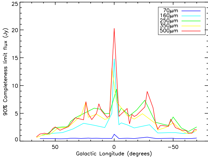
Fig. 9. Ninety percent completeness limits in flux density for a population of sources with the same distribution of sizes as the one extracted by CUTEX as a function of Galactic longitude. The significant increase in the completeness limit in the inner Galaxy and especially close to the Galactic centre is due to the brighter background emission in such regions.
