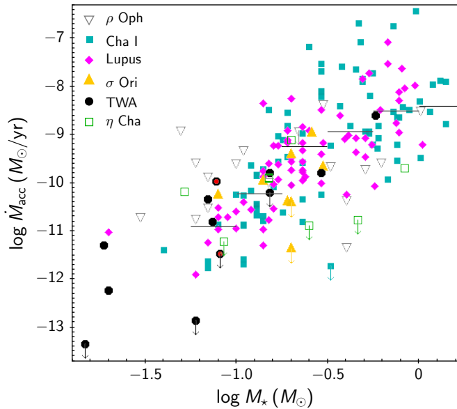
Fig. 11. Comparison between the \dot{M}_{\text{acc}} - M_* distributions obtained from X-shooter data for \rho Ophiuchi, Lupus, Chamaeleon I, \sigma Orionis, TWA, and \eta Chamaeleontis (symbols and sources of data as detailed in the caption of Fig. 10). Upper limits in \dot{M}_{\text{acc}} are marked by downward arrows. The horizontal lines mark the median \dot{M}_{\text{acc}} measured in bins of 0.25 dex in \log M_* for the combined Cha I and Lupus datasets.
