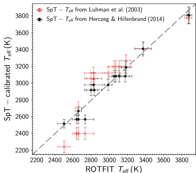
Fig. 3. Comparison between the T_{\text{eff}} estimates derived with ROTFIT for all targets and spectra, and the T_{\text{eff}} corresponding to the SpT estimated for each source (Table 2) using the calibrations of Luhman et al. (2003, red symbols) and of Herczeg & Hillenbrand (2014, black symbols). The x -axis uncertainties are those derived from the fit; the y -axis uncertainties correspond to half the difference in T_{\text{eff}} between consecutive spectral subclasses in the corresponding SpT– T_{\text{eff}} scale. The identity line is dashed in gray to guide the eye.
