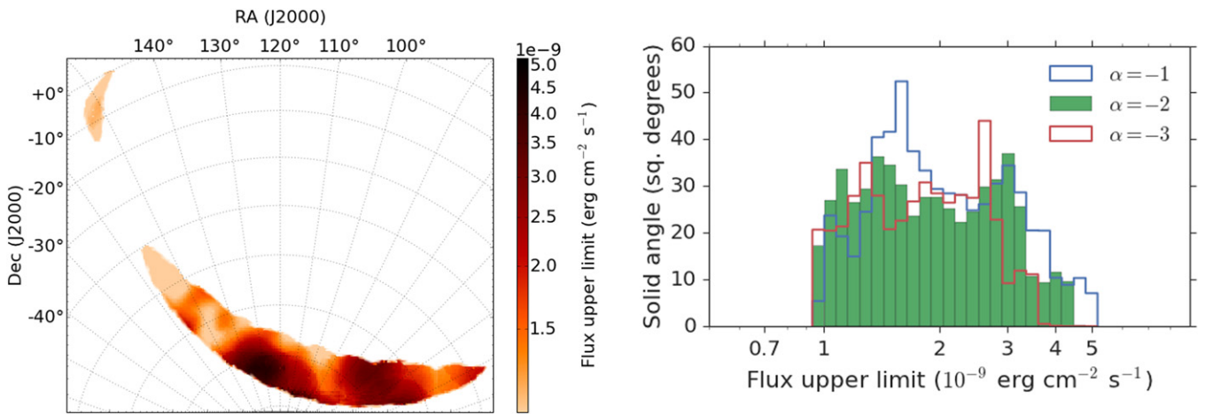
Figure 2. Flux upper limits (95% c.l.) in the energy range 100 MeV–1 GeV for GW150914 during the interval T_1 (4442–4867 s from t_{\text{GW}} ). Left panel: the upper limits map covering the 90% region of the LIGO probability map. Right panel: the histogram of the upper limits in the map. We assumed a power-law spectrum for the source, with a photon index \alpha of -2 (typical of afterglows of GRBs; green histogram), -1 (blue histogram), and -3 (red histogram). While the distributions are slightly different for the three cases, the ranges spanned by the upper limits are largely independent of the photon index.
