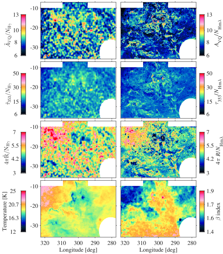
Fig. 11. Three upper rows: spatial variations of the dust properties per gas nucleon with the total gas measured by N_{\text{H}\gamma} on a 0.375 pixel grid (left) and by N_{\text{Hml}} on a 0.125 pixel grid (right). Lower row: colour temperature and \beta index of the dust SED, measured at 5' resolution by Planck Collaboration XI (2014) and displayed on a 0.125 pixel grid. The A_{VQ}/N_H values are in units of 10^{-22} mag \text{cm}^2 , \tau_{353}/N_H in 10^{-27} \text{cm}^2 , and 4\pi R/N_H in 10^{-31} W.
