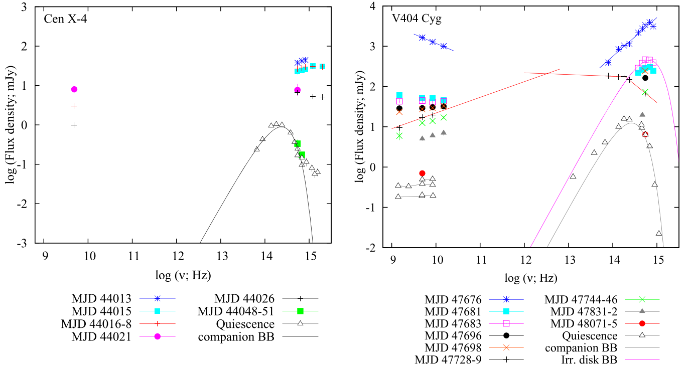
Figure 2. Left panel: broadband, radio to optical (dereddened) spectra of Cen X-4 during its 1979 outburst and quiescence. The black line is a blackbody with a temperature of 4050 K representing the companion star. Data are from Blair et al. (1984), Bernardini et al. (2013), Canizares et al. (1980), Hjellming (1979), Kaluzienski et al. (1980), Shahbaz et al. (1993), van Paradijs & McClintock (1994), and Wang & Wang (2014). Right panel: broadband, radio to optical (dereddened) spectra of V404 Cyg during its 1989 outburst and quiescence. The first spectra were obtained near the peak of the outburst, and in general, time progresses from top to bottom. The red lines show the fit to the jet spectrum obtained on MJD 47,728–29 (Russell et al. 2013), and the gray and purple curves show single-temperature blackbody approximations to the data in quiescence and on MJD 47,683, respectively. The radio data are taken from Han & Hjellming (1992), Gallo et al. (2005), and Hynes et al. (2009); the gray lines joining radio data points are taken on the same dates. The infrared, optical, and UV data are from Gehrz et al. (1989a, 1989b), Casares et al. (1991, 1993), Leibowitz et al. (1991), Udalski & Kaluzny (1991), Wagner et al. (1991), Han & Hjellming (1992), and Hynes et al. (2009).
