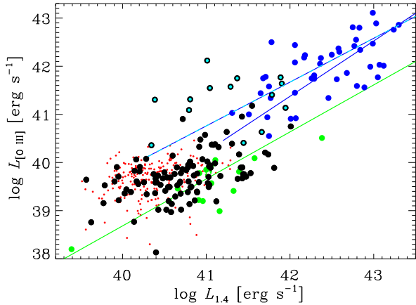
Fig. 4. Radio (NVSS) vs. [O III] line luminosity of the FRIICAT (black), FRICAT (red), 3C-FR I (green), and 3C-FR II samples (blue). The green line (blue) shows the linear correlation between these two quantities derived from the FR Is (FR IIs) of the 3C sample from (Buttiglione et al. 2010). The dashed blue-cyan line is instead the linear fit on both the 3C and the FRIICAT HEGs.
