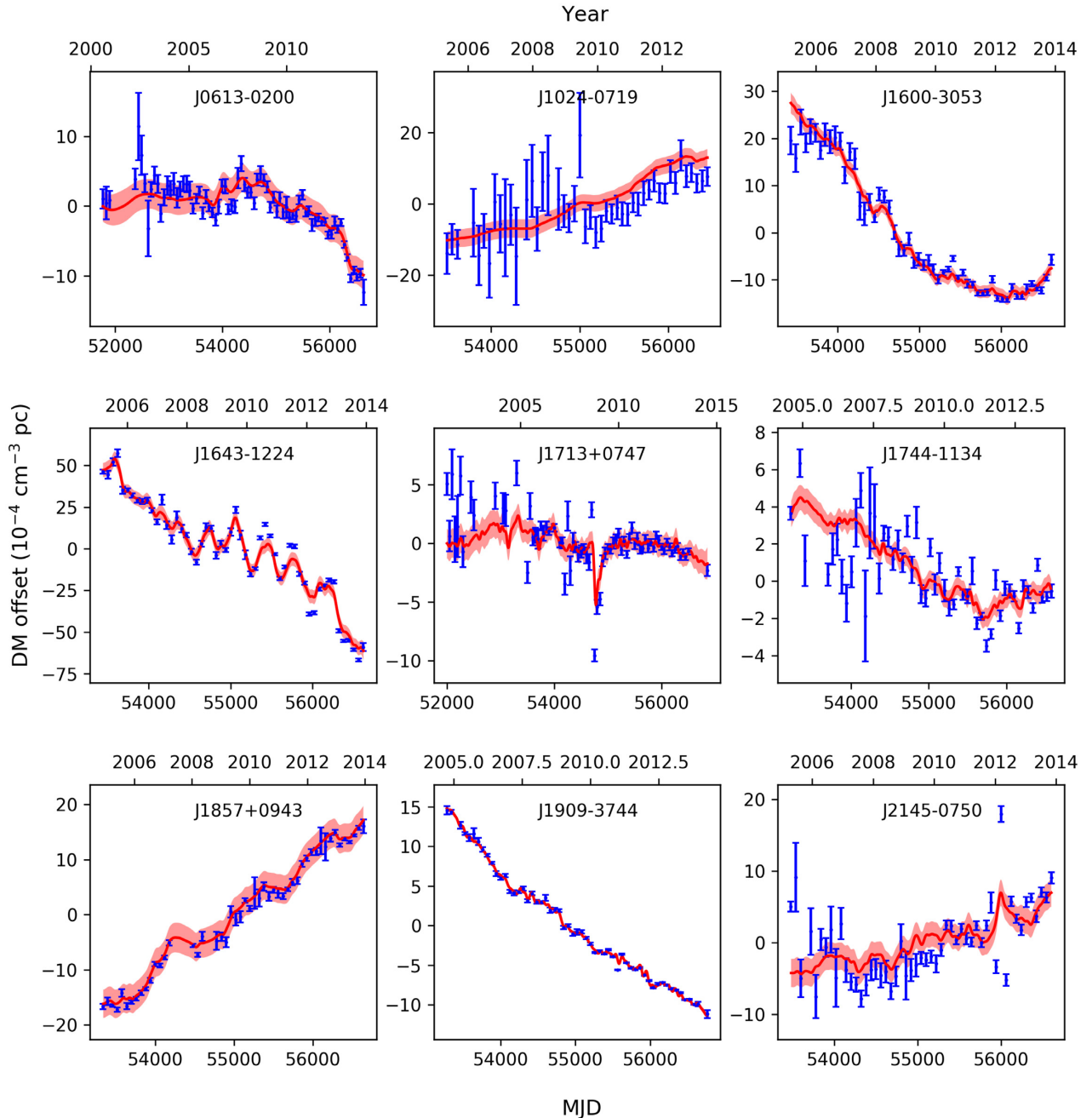
Figure 3. The time-dependent DM variations for pulsars that are observed by all three PTAs obtained using the DMMODEL ( blue ) as described in VersionA (see Section 4.1). Note that the mean DM is subtracted and only the variation is plotted. For comparison, the DM variations obtained using the power-law model described in VersionB (see Section 4.2) are overplotted ( red ), and their uncertainties are estimated using a Gaussian process regression method. The overall features in DM variations obtained from the two versions are consistent with each other within their measured uncertainties. Note that we omitted PSR J1939+2134 in this figure because of its complicated timing noise behaviour.
