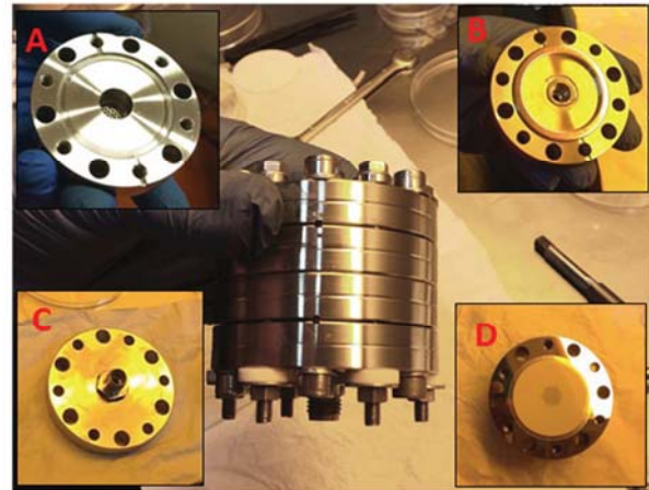
Fig. 6. Assembled experimental cell and assembly parts: (A) internals of the inner flange with view of perforated grid and solid zinc slot; (B) installation of the copper ring gasket on the internal face of outer flange; (C) external face of outer flange, (D) placement of the membrane on the external face of inner flange.
