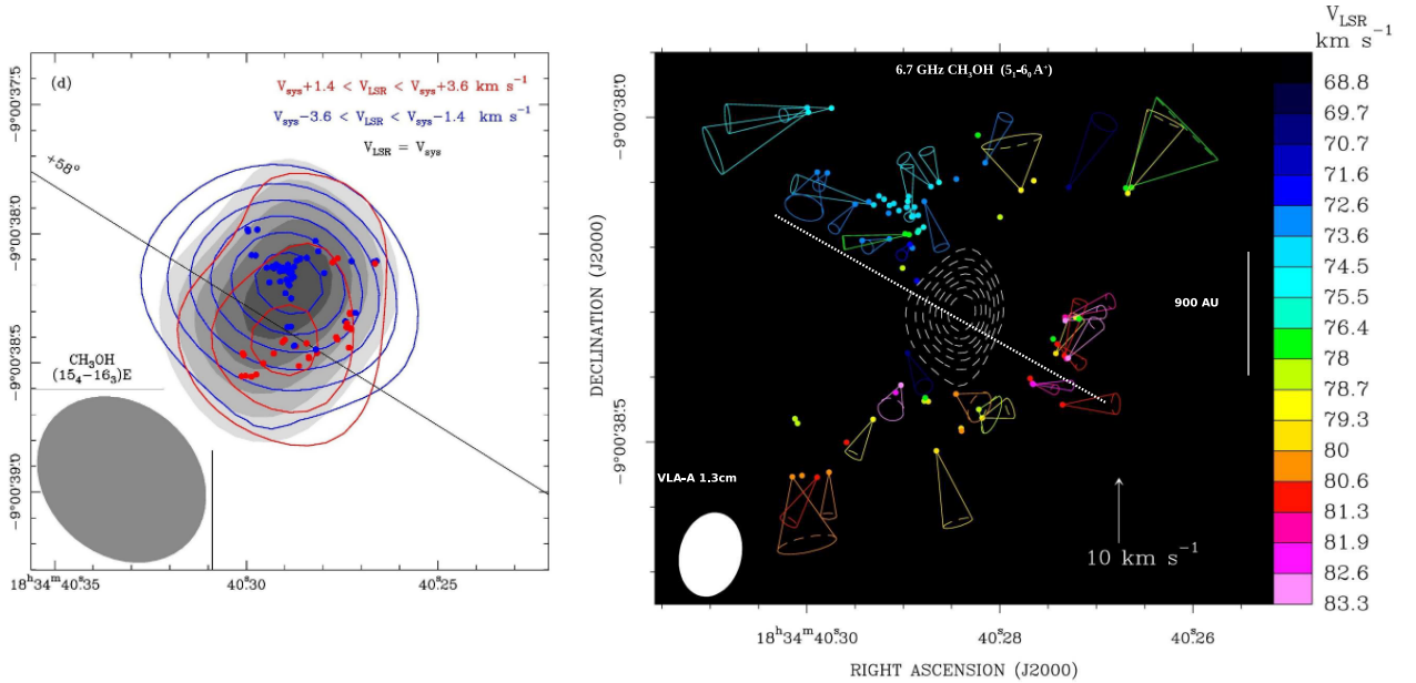
Figure 3: Left Panel) Map of the \text{CH}_3\text{OH} ( 15_4-16_3 )E line emission observed with the SMA towards G23.01-0.41 by [12], with gray, blue, and red contours representing, respectively, the systemic velocity, and the blue- and redshifted wings of the line. Blue and red dots mark the positions of the blue- and redshifted methanol maser spots. Right Panel) Positions and proper motions ( colored dots and cones , respectively) of the 6.7 GHz methanol masers derived with multi-epoch VLBI observations, and VLA 1.3 cm continuum ( dashed contours ) [13].
