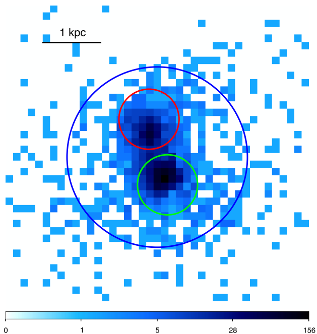
Figure 1. Chandra image of the central ( 10 \times 10 arcsec ^2 ) region of NGC 6240 in the 5–7.5 keV band (rest frame), obtained by combining the ACIS-S observations of 2001 July (ObsID 1590) and 2011 May (ObsID 12713). Subpixel resolution by a factor of 2 is adopted, so one pixel in this figure has a physical size of 126 pc. The regions employed in the spatially resolved spectral analysis are also shown: northern nucleus (red), southern nucleus (green) and diffuse Fe K emission (blue).
