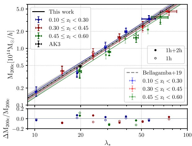
Figure 7. Mass-richness scaling relation for the full catalogue (black) and for the low (blue), intermediate (red), and high (green) redshift bins. The thick line corresponds to the model formulated in equation (36). Full and empty data points represent the measurements over the whole radial profile and over the central region of the halo, respectively. We compared our results with those presented in Bellagamba et al. (2019). The fainter colored points represent the data and the dashed lines represent the model. The relative change with respect to the results of this work is displayed in the bottom panel.
