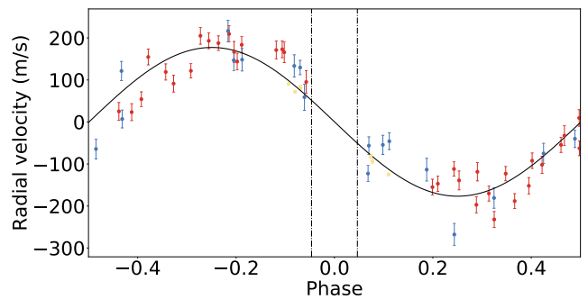
Fig. 1. Radial velocities of WASP-121b, phase-folded with the orbital period and detrended from stellar activity. Coralie data points have been obtained before (red) and after (blue) the fiber upgrade ( Ségransan et al. 2010 ). HARPS datapoints are shown in gold. Our best-fit Keplerian model to the out-of-transit data is shown as a solid black line (datapoints obtained in the frame of transit observations were binned, see text). The first and fourth transit contacts are indicated by dash-dotted vertical black lines.
