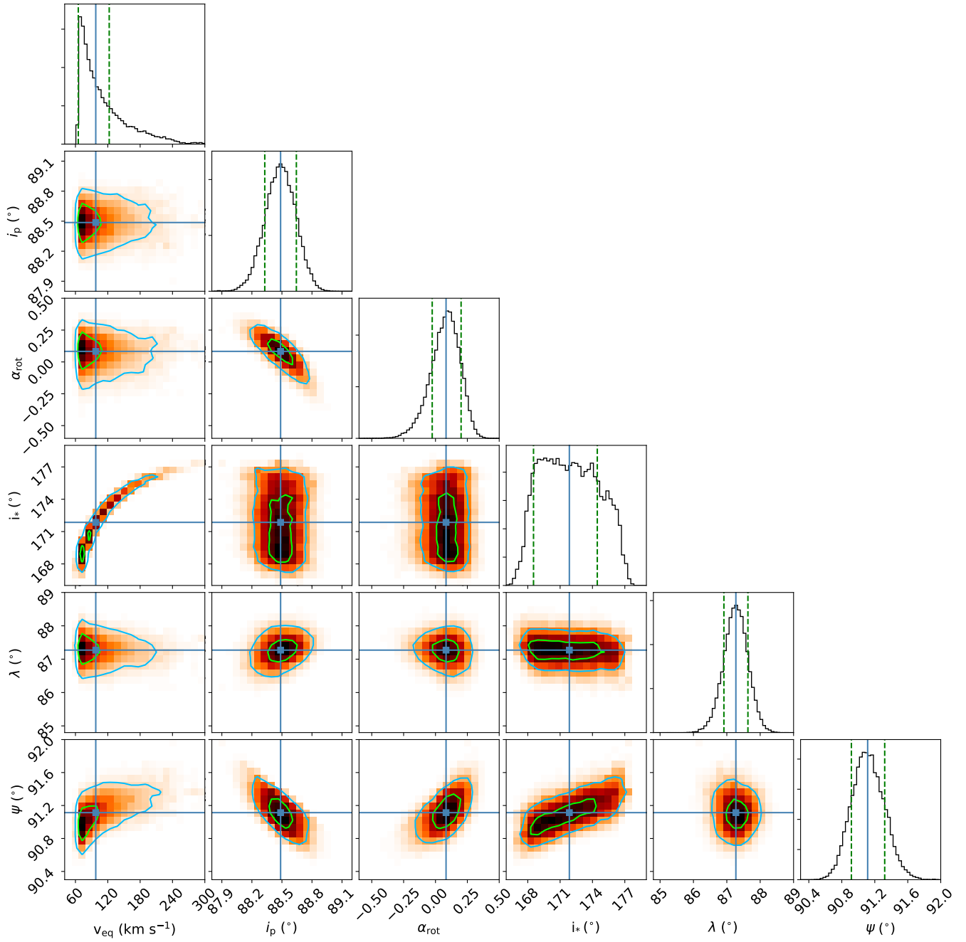
Fig. B.2. Same as in Fig. B.1, with samples limited to the region with high stellar inclination.
