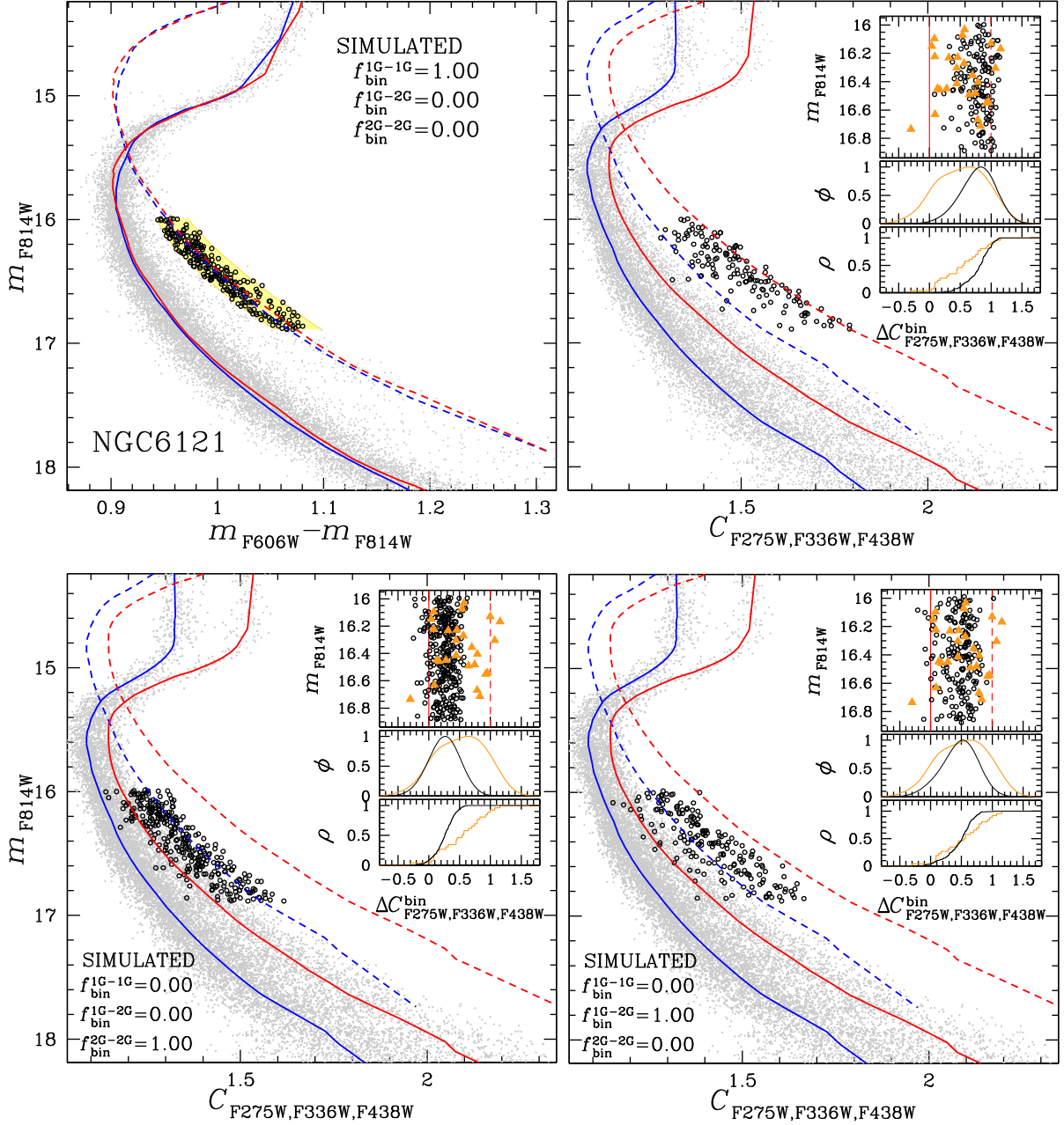
Figure 5 Upper panels show the simulated m_{F814W} versus m_{F606W} - m_{F814W} CMD (left) and m_{F814W} versus C_{F275W, F336W, F438W} diagram (right) where we assumed that all the binaries are formed by pairs of 1G stars. The yellow region includes all the selected binaries. The inset compares the m_{F814W} versus \Delta C_{F275W, F336W, F438W}^{bin} diagram for the selected sample of simulated (black circles) and observed (orange triangles) binaries and the corresponding \Delta C_{F275W, F336W, F438W}^{bin} kernel distributions and cumulative distributions. In the bottom panels, we assumed that all the binaries are formed by pairs of 2G stars (left) and by pairs of 1G and 2G stars (right). Simulated stars are coloured grey, while the selected simulated binaries are marked with black circles.
