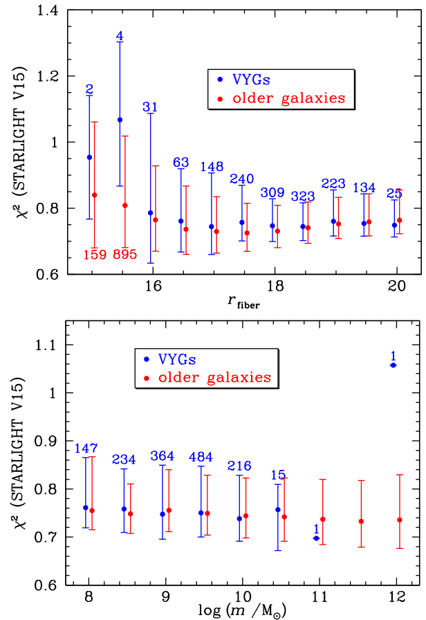
Figure 13. Spectral fit quality (reduced \chi^2 ) for the STARLIGHT V15 fits on the complete sample, as a function of the fiber magnitude (proxy for the signal to noise of the spectrum, top) and of the galaxy stellar mass (bottom), for both the VYGs (blue) and the older galaxies (red). The symbols denote medians, while the error bars represent 16th and 84th percentiles. The numbers above the error bars indicate the number of VYGs per bin.
