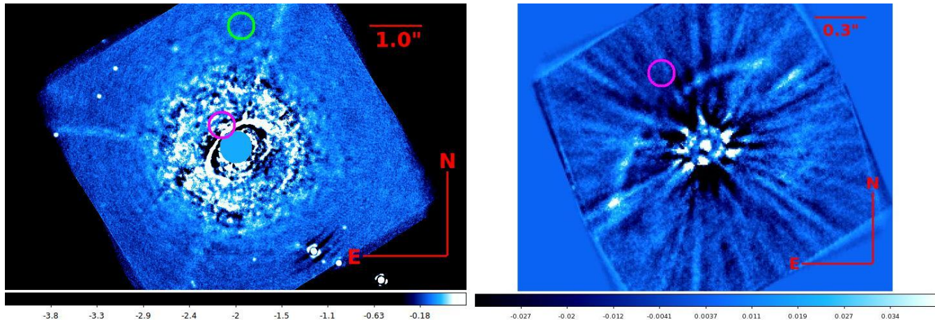
Figure 1. Final images obtained from the 2018-05-06 observations. In both cases the values are expressed in counts. Left: IRDIS final image obtained applying the PCA algorithm and subtracting 1 mode from the original data. The green circle is to enlight the zone around the planet proposed by Pinte et al. (2018) , the magenta circle enlight the zone of the planet proposed by Guidi et al. (2018) . The mask covering the star has a radius of 0.37'' . Right: IFS final image obtained using the PCA algorithm subtracting 1 mode from the original data. As for the IRDIS image, the magenta circle identify the zone around the planet proposed by Guidi et al. (2018) .
