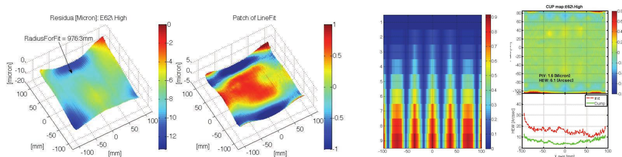
Figure 11: (A) Overall residuals with respect to the theoretical reference cylinder of 1m radius of curvature. (B) The simplified-model starting map assumes only longitudinal profile errors, neglecting azimuthal residual curvature and tilts. (C) The corrective damping map to be applied in Fourier space: according to the wavelength and to the relative position with respect to the rib, the corrective factors can be more or less effective. (D) The damped maps according to the simplified model and the corresponding results.
