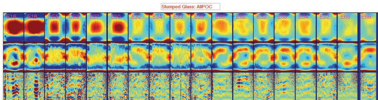
Figure 13: The slumped glass metrology before integration of the last PoCs. E16 and E18 have been integrated in the PoC#3. From CE5 to E35, the segments have been used for the PoC#4. From R60 to E68, the glass have been integrated in the PoC5d.
