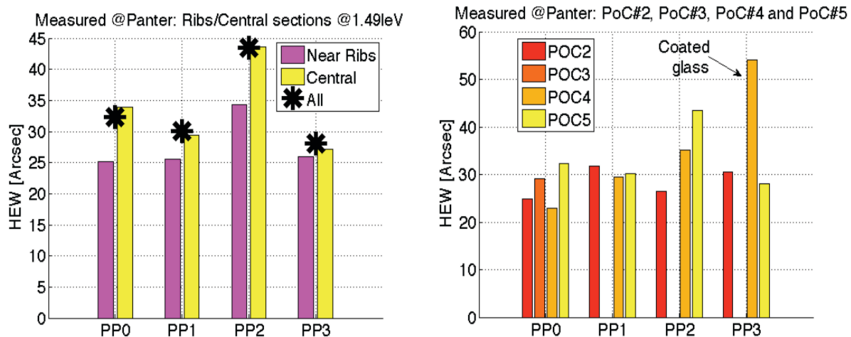
Figure 18: (A) HEW of the different layers of the PoC#5d with a dashed and a complementary mask: the HEW is evaluated in correspondence of the ribs (magenta) and of the portion of the glass between the ribs (yellow). In black the HEW of the complete PP. (B) The HEW of each PP at its best focus. Colours (from red to yellow) refer to the different prototypes (PoC#2, PoC#3, PoC#4 and PoC#5d). The PoC#4 PP3 was a dummy layer integrated for test the integration procedure with coated glasses.
