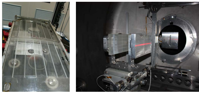
Figure 1: Measurement configuration @Panter/MPE for the PoC#5d and the WP1, measured end of June 2016. The two prototypes are supported independently on the same flange so that they can be measured one after the other without interrupting the vacuum chamber configuration.
