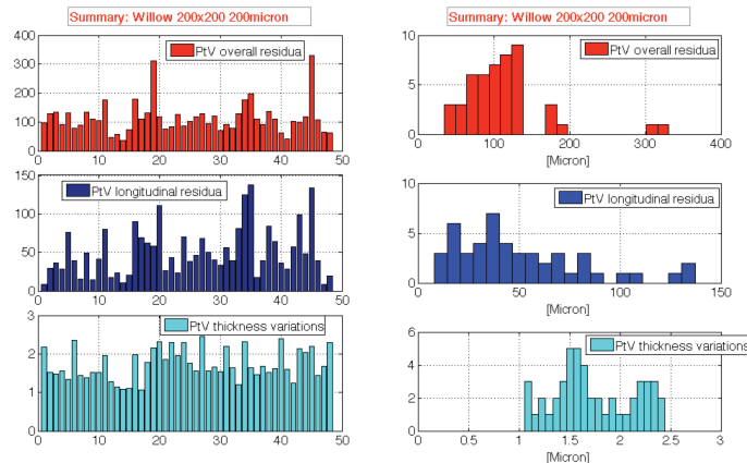
Figure 28: (A) The overall PtV of the flatness error of the different glass sample. (B) The longitudinal PtV of the flatness error of the different glass samples. (C) The PtV of the thickness variation maps.
