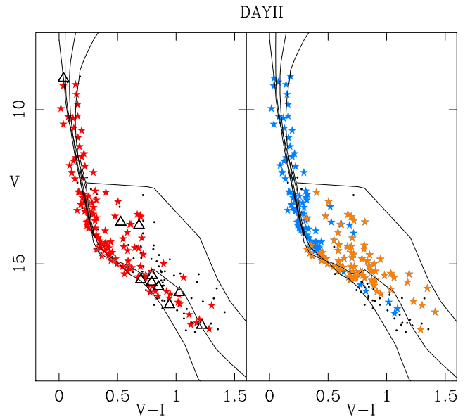
Figure 6. Distribution in the CM diagram V, (V - I) of stars with and without kinematic membership assignments, and comparison to their selection as photometric candidate members. In both panels, stars with GES data in the optical FOV are plotted. The left-hand panel shows as red stars those selected as kinematic members, and as black triangles those rejected as outliers. The right-hand panel shows those among them selected as photometric MS+post-MS, and PMS members, marked respectively in blue and orange colours. The ZAMS and isochrones are plotted as in Fig. 4.
