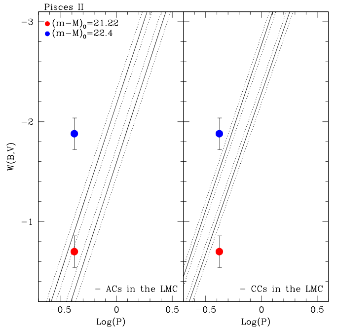
Figure 13. PW relations (solid lines) for ACs (left panel; from Ripepi et al. 2014) and CCs (right panel; from Jacyszyn-Dobrzaniecka et al. 2016) in the LMC, transformed to the B and V bands. Dotted lines represent the 1\sigma uncertainties, which for the AC relations correspond to 0.15 mag and for the CCs to 0.10 mag. A red filled circle shows the position of V4, according to the period of \sim 0.42 days and a Wesenheit index calculated for a distance modulus of (m - M)_0 = 21.22 mag as estimated from V1, the RRL inside the half-light radius of Psc II. The blue filled circle shows V4 but adopting a mass of 1.8 M_\odot and a Wesenheit index calculated for a distance modulus of 22.4 mag.
