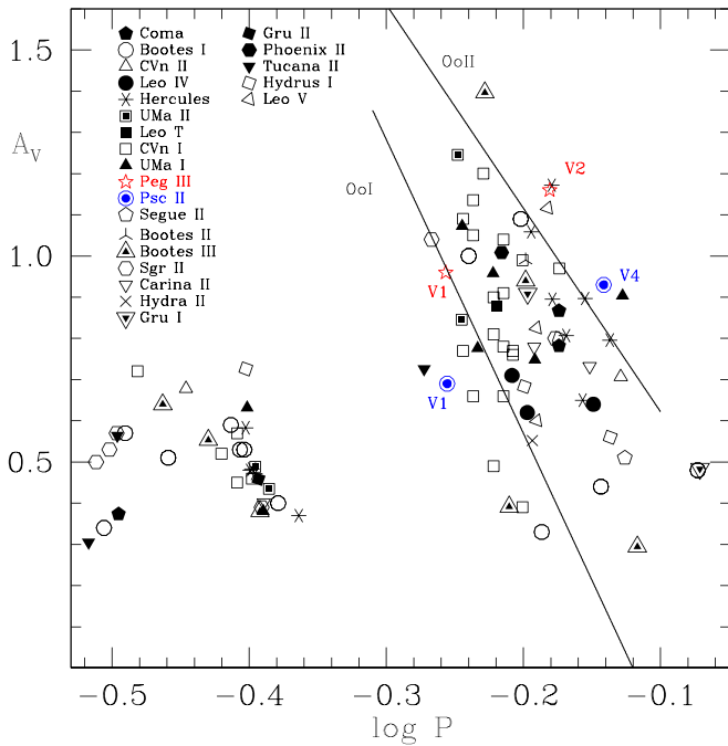
Figure 5. Period–amplitude (Bailey) diagram: the bona fide RRL star inside the r_h of Psc II (star V1) and the variable star with uncertain classification, V4 (plotted adopting the same period as RRLs, P = 0.722 days), are shown as blue circles, while the bona fide RRL in Peg III, V1, and a variable star with uncertain classification, V2 (assuming the same period as RRLs, P = 0.6594 days), are marked by red stars. Solid lines show the loci of Oo I and Oo II Galactic GCs according to Clement & Rowe (2000). For comparison, we have also plotted the RRLs identified in 21 other MW UFDs (see text for details). We have transformed the SDSS g -band amplitudes, A_g , of the RRLs in Gru I, Gru II, and Phoenix II to V -band amplitudes, A_V , using a constant ratio, A_g/A_V = 1.2 , according to Marconi et al. (2006, see their Figures 11 and 12). The Gaia G -band amplitudes of the RRLs in Bootes I and III, Coma Berenices, Hydra I, Tucana II, and UMa II reported in Vivas et al. (2020) were converted to A_V amplitudes using Equation (3) in Clementini et al. (2016).
