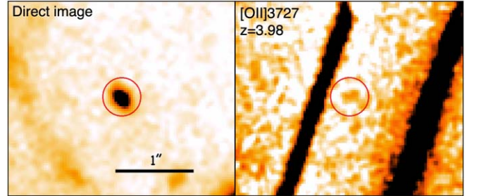
Figure 3. The direct image of image 3c (NIRISS/CLEAR; left) and the detection of [OII] \lambda 3727, 3729 despite nearby contamination from other galaxies. The redshift of image 3c is consistent with the counterimages 3a and 3b.
