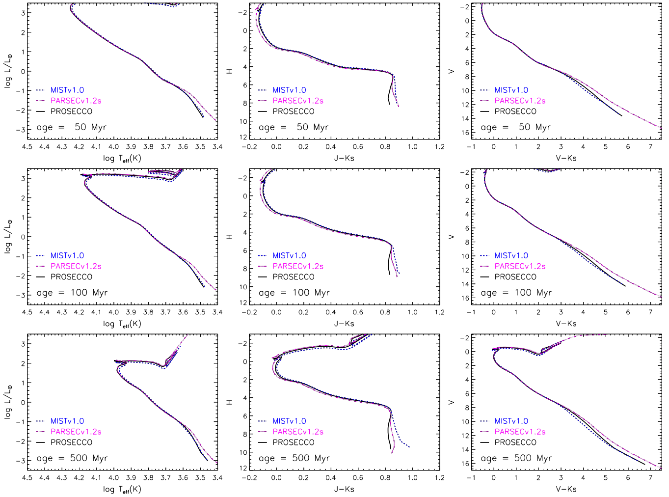
Fig. A.1. Comparison among 50, 100 and 500 Myr isochrones from the selected sets in the HR diagram and in various CMDs. MISTv1.0 = MESA isochrones by Choi et al. (2016); Dotter (2016), PARSECv1.2s = PARSEC isochrones in the PARSEC 1.2S version (Chen et al. 2014), PROSECCO = isochrones specifically calculated for the present work; see text.
