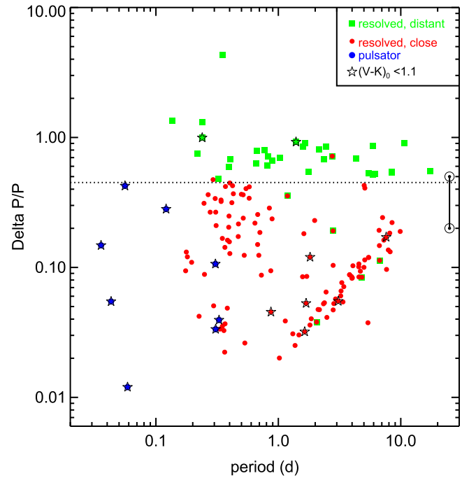
Figure 15. Plot of \Delta P/P_1 vs. P for pulsators (blue circles), resolved distant peaks (green squares), and resolved close peaks (red circles). An additional black star indicates that those stars have (V - K_s)_0 \leq 1.1 (see Paper III). The range of possible values for the Sun is included for reference ( \odot ); if one takes as \Delta P the range of periods measured where sunspots occur, \Delta P/P_1 \sim 0.1 – 0.2 , but if one takes the full range of \Delta P , equator to pole, \Delta P/P_1 \sim 0.5 . The dotted line is at \Delta P/P_1 = 0.45 and denotes the boundary between close and distant resolved peaks. Some objects are tagged as both close and distant peaks (e.g., there are at least three periods in these objects, two of which are close and a third of which is not close). Pulsators ( \delta Scutis) are largely outliers. The linear feature in the lower right predominantly becomes the slow sequence found in the P vs. (V - K_s)_0 plot. The clump of sources near P \sim 0.4 and \Delta P/P_1 \sim 0.3 becomes the M star fast sequence in the P vs. (V - K_s)_0 plot. The lack of sources below the linear feature is largely an observational bias.
