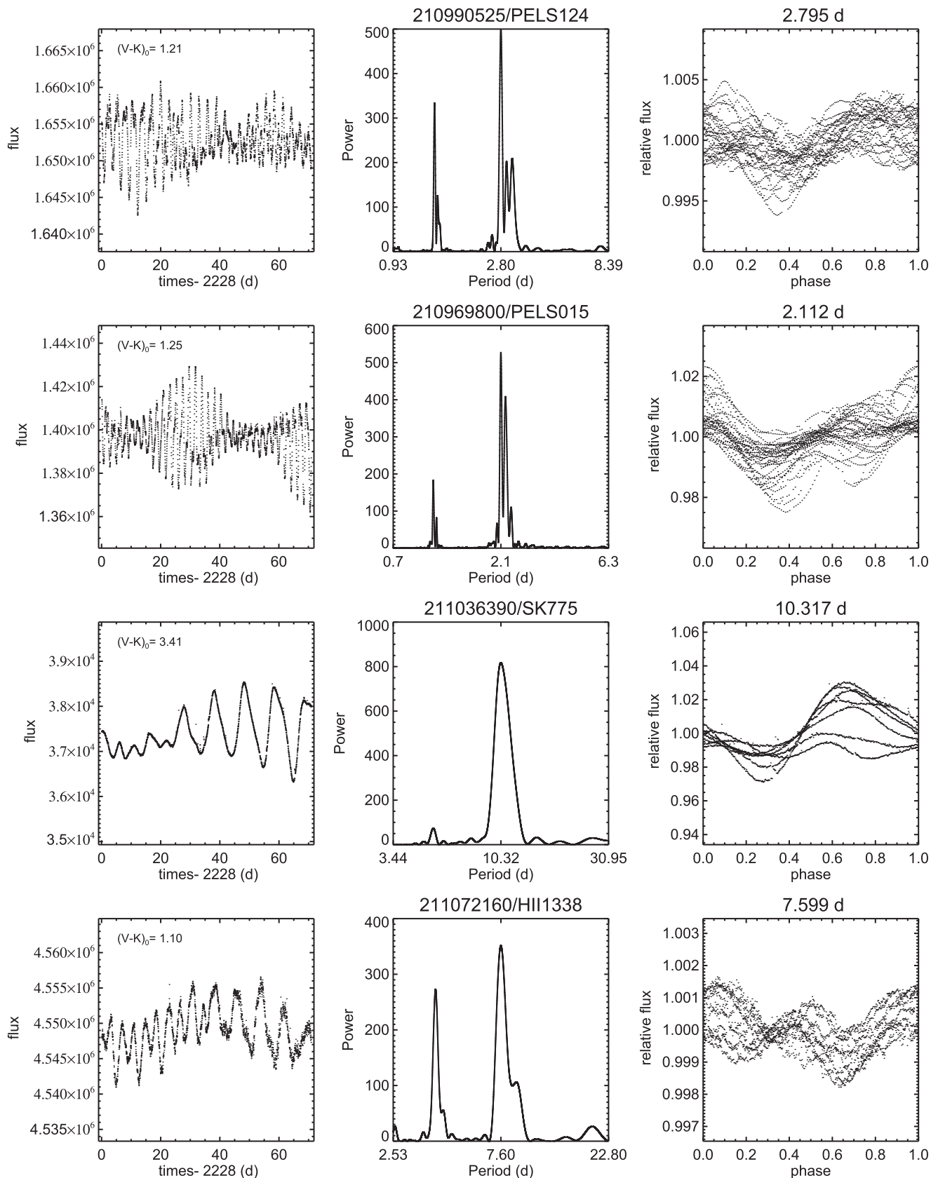
Figure 3. Four examples of the beater and complex peak categories. Beating is seen in the LC, and for these examples, the peak in the periodogram is complex, broad, and/or structured. Left column: full LC (with (V - K_s)_0 for star as indicated); middle column: periodogram; right column: phased LC for maximum peak. Rows, in order (with the periods corresponding to significant peaks in parentheses): 210990525/PELS 124 (2.795, 1.421, 3.330), 210969800/PELS 015 (2.112, 2.212), 211036390/SK 775 (10.317), and 211072160/HII 1338 (7.599, 8.899). Note that the power spectrum shows peaks of measurable width and/or multiple peaks. Sometimes the multi-peaked structure can be found in both the main peak and its harmonic. These LCs are likely a result of latitudinal differential rotation and/or spot evolution.
