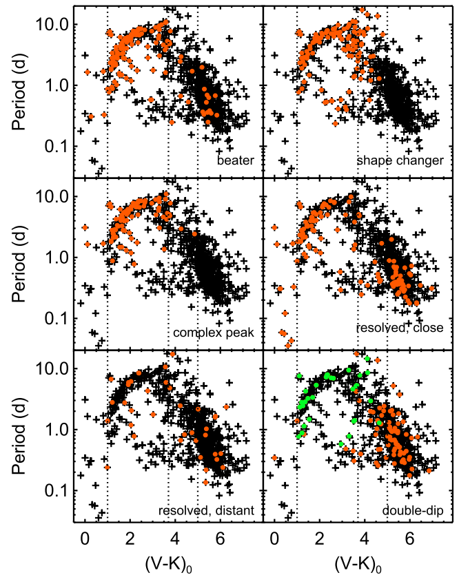
Figure 14. Plot of P vs. (V - K_s)_0 , highlighting several of the LC categories described in the text. Notation (and the location of the dotted vertical lines) is the same as in Figure 13. The slow sequence consists of beaters, shape changers, complex peaks, and resolved close peaks. Resolved close peaks are also found in the fast sequence, and these are largely the photometric binaries from Figure 12. Some beaters and resolved distant peaks are also photometric binaries. The double-dip LCs above are found throughout this diagram, but those showing movement within the campaign are distinctly higher mass.
