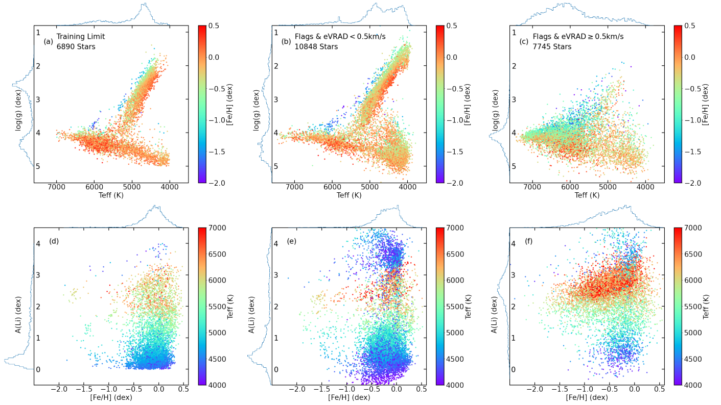
Fig. 11. Results for the observed sample. Top row: Kiel diagram for the observed sample stars with S/N > 10 dex and labels within training limits color-coded with [\text{Fe}/\text{H}] . (b) Same plot as (a) but for stars with S/N > 10 pix, GES-iDR6 flags and E\_VRAD < 0.5 \text{ km s}^{-1} . (c) Same selection as (b) but for E\_VRAD \geq 0.5 \text{ km s}^{-1} . Each subplot shows a histogram of the labels on the left and top axis. Bottom row: A(\text{Li}) vs. [\text{Fe}/\text{H}] color-coded with T_{\text{eff}} for the same stars as the Kiel diagram on top.
