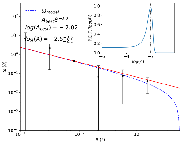
Figure 8. TPCF and fits for All MLAGN (top panel), MLAGN with z < 1 (middle panel) and MLAGN with z \geq 1 (bottom panel). The left panel shows the TPCF, the red solid line represents the power law best fit to \omega(\theta) and the dashed blue line is the same as the red line but with the integral constraint, \sigma^2 subtracted from it. The inset in the top right corner shows the probability density function for the value of A to fit the TPCF, with the dashed line showing the best fit value. The right panel shows the corresponding P.D.F. for r_0 .
