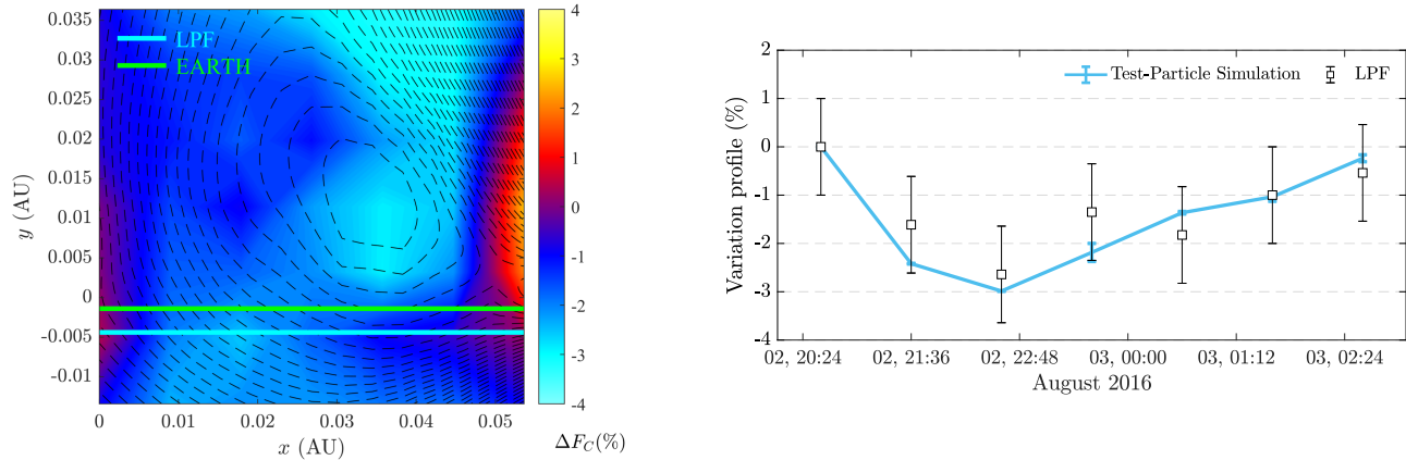
Figure 6. Left: Proton fluence percentage variation obtained from equation (5) in the energy interval 70 MeV - 100 GeV. The black dashed lines are the level curves of the potential vector A(x, y) . The cyan (green) solid line is the LPF (Earth) path through the MC. Right: Comparison between the LPF observations and the fluence variation profile obtained from the simulation with standard errors.
