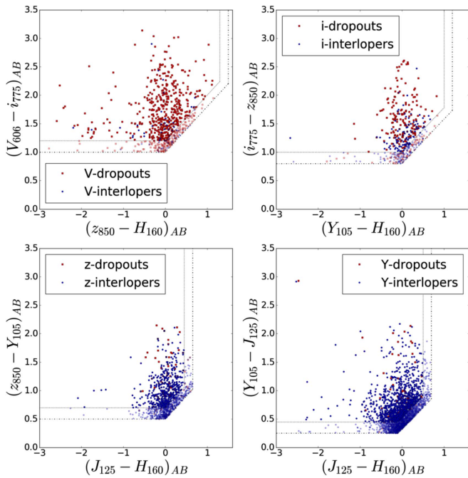
Figure 12. Color–color selection box used to identify V_{606} - (upper left), i_{775} - (upper right), z_{850} - (bottom left) and Y_{105} -dropouts (bottom right), following the color selection presented in Bouwens et al. (2015). Red squares represent dropouts, i.e., high- z sources with no flux blueward of the Lyman-break; blue circles represent interlopers, i.e., high- z candidates showing a detection in the blue bands. Dashed lines represent the boundaries of the original sample selection, following Bouwens et al. (2015); dashed–dotted lines represent the boundaries of the enlarged sample (see the text for details). Darker symbols refer to the original selection, lighter ones refer to the enlarged selection.
