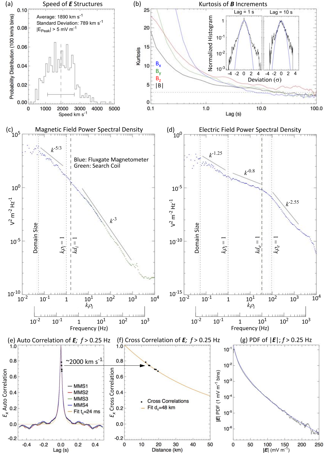
Figure 3. Properties of E and B in strong turbulence. (a) Histogram of the speed of E structures; E is filtered to frequencies > 0.25 \text{ Hz} . A velocity is determined from time delays between 4 s intervals that are calculated via cross-correlation. Events with a high correlation coefficient ( > 0.8 ) and amplitudes greater than 5 \text{ mV m}^{-1} are used to make the histogram. The directions are nearly random. The average speed is 1890 \text{ km s}^{-1} . (b) Kurtosis of increments of B as a function of lag time. The colors represent components. The kurtosis relaxes to 3 (Gaussian distribution) at greater than \sim 10 \text{ s} lag. Distributions at 1 and 10 s lag are included in the plot. (c) PSD of B as a function of |k|\rho_i and frequency (lower axis). The PSD is calculated as a function of frequency using a pseudo log-spaced FFT algorithm and translated to a function of |k|\rho_i ( \rho_i is given in the table in Figure 1) assuming a structure speed of 1890 \text{ km s}^{-1} . The vertical dashed lines show the domain size ( 10^8 \text{ m} ), |k|\rho_i = 1 , and |k|d_i = 1 . The solid black lines are for visual reference; they are not fits. (d) PSD of E as a function of |k|\rho_i and frequency (lower axis). The PSD is calculated with the same algorithm used for the PSD of B . The vertical dashed lines show the domain size ( 10^8 \text{ m} ), |k|\rho_i = 1 , |k|d_e = 1 , and |k|\rho_e = 1 . The solid black lines are for visual reference; they are not fits. (e) Autocorrelation of E_x (8192 samples s -1 and filtered to f > 0.25 \text{ Hz} ) as a function of lag time. The colors represent the four spacecraft. The gold line represents a fit to an exponential ( e^{-t/t_c} ) with t_c = 24 \text{ ms} . (f) Expanded view (six black dots) of the cross-correlation E_x ( f > 0.25 \text{ Hz} ) between each of the spacecraft. The distances between the spacecraft are given in Figure 1(j). The gold line is an exponential with a correlation distance of 48 \text{ km} . (g) PDF of |E| for f > 0.25 . The PDF fits remarkably well to a stretched exponential, e^{-\sqrt{|E|/E_0}} , where E_0 = 1.3 \text{ mV m}^{-1} .
