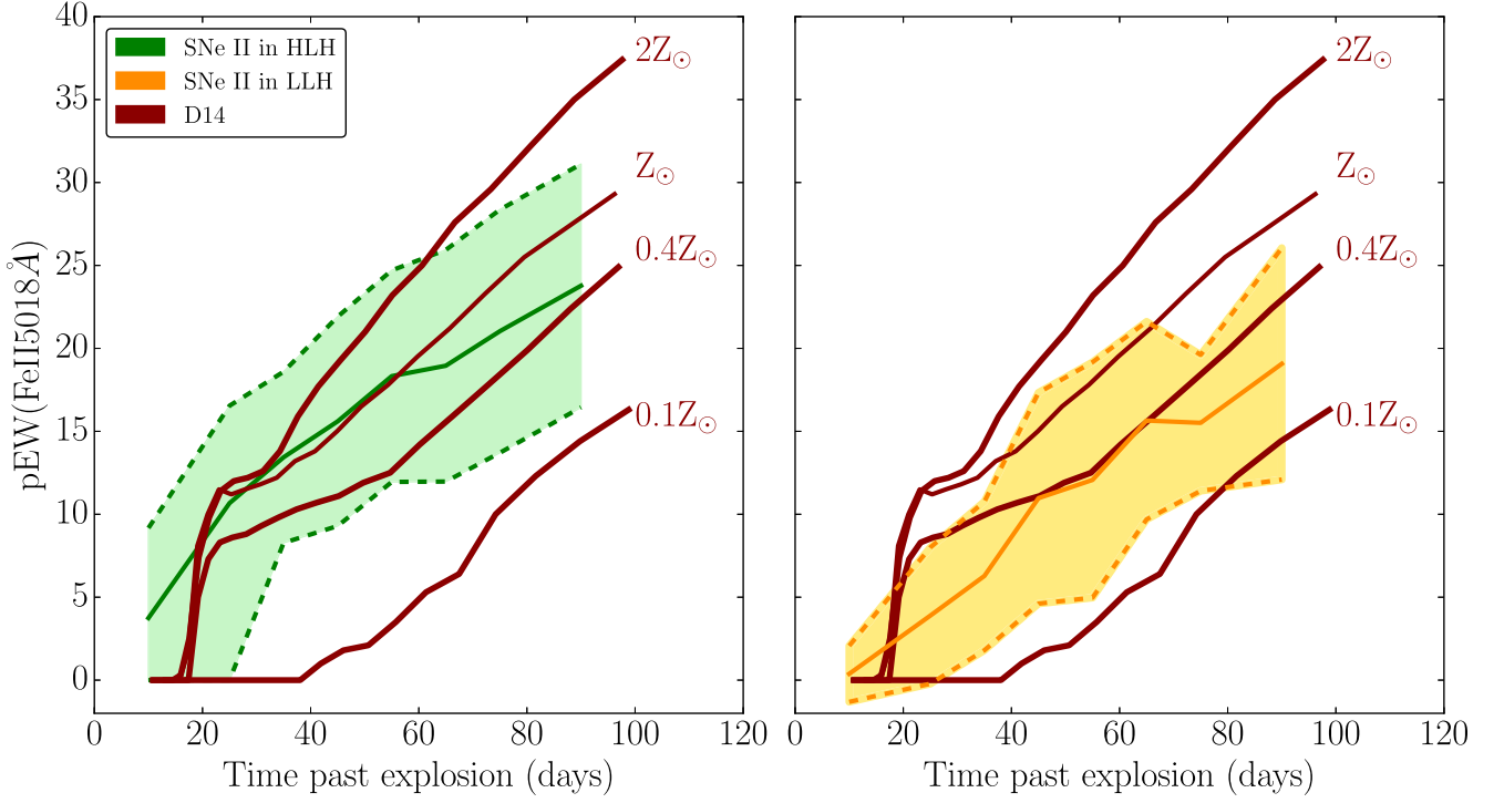
Figure 6. Temporal evolution of pEW(\text{Fe II } 5018 \text{ \AA}) from explosion to +90 d, in both the data and models at four different metallicities. The observational data are binned in time. Left: Comparison between the SNe II in high-luminosity hosts. The green solid line represent the mean of the pEW within each time bin, while the dashed green lines indicate the standard deviation. Right: The comparison with SNe II in low-luminosity hosts, with the mean of the pEW orange solid line and the standard deviation in dashed orange lines. In both panels, the brown solid lines represent the D14 models as labelled.
