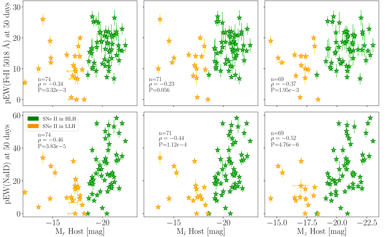
Figure 7. Correlations between pEW(\text{Fe II } 5018 \text{ \AA}) (upper panels) and pEW(\text{Na I D}) (lower panels), and the galaxy absolute magnitudes: M_r (left), M_i (centre), and M_z (right). Green stars represent SNe in high-luminosity hosts, while yellow stars are SNe II in low-luminosity hosts. In each panel, n is the number of events, \rho is the Pearson's correlation coefficient, and P is the probability of detecting a correlation by chance.
