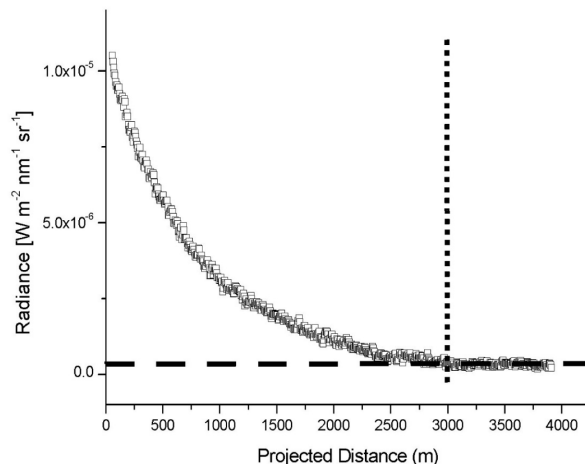
Figure 6. An example of how the leading edge determined from the difference image on 2015 September 10 (20:51:22.797) is used to derive the expansion velocity (left panel). A radial brightness profile (right panel) is an averaged value outwards from the nucleus in the selected box marked in the difference image. The subtracted background level is shown by the dashed line. The cross match in between the radial brightness profile and subtracted background level is shown by the vertical dotted line.
