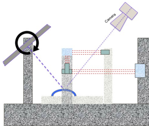
Fig. 3. Side view of the new metrological device.
