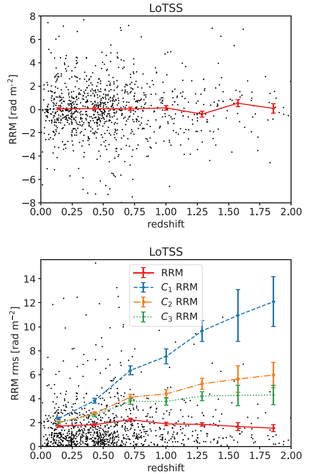
Figure 4. Top panel: mean of the RRM sample selected from the LoTSS RM catalogue in equal-width redshift bins (red solid line). Individual RRMs are also shown (dots). Bottom panel: as for the top panel but for the RRM rms deviation (red solid line). The rest-frame \text{RRM}_0 corrected for the redshift effects C_1 (dashed line), C_2 (dot-dashed line), and C_3 (dotted line) are also plotted. Individual |\text{RRM}| s are shown as dots.
