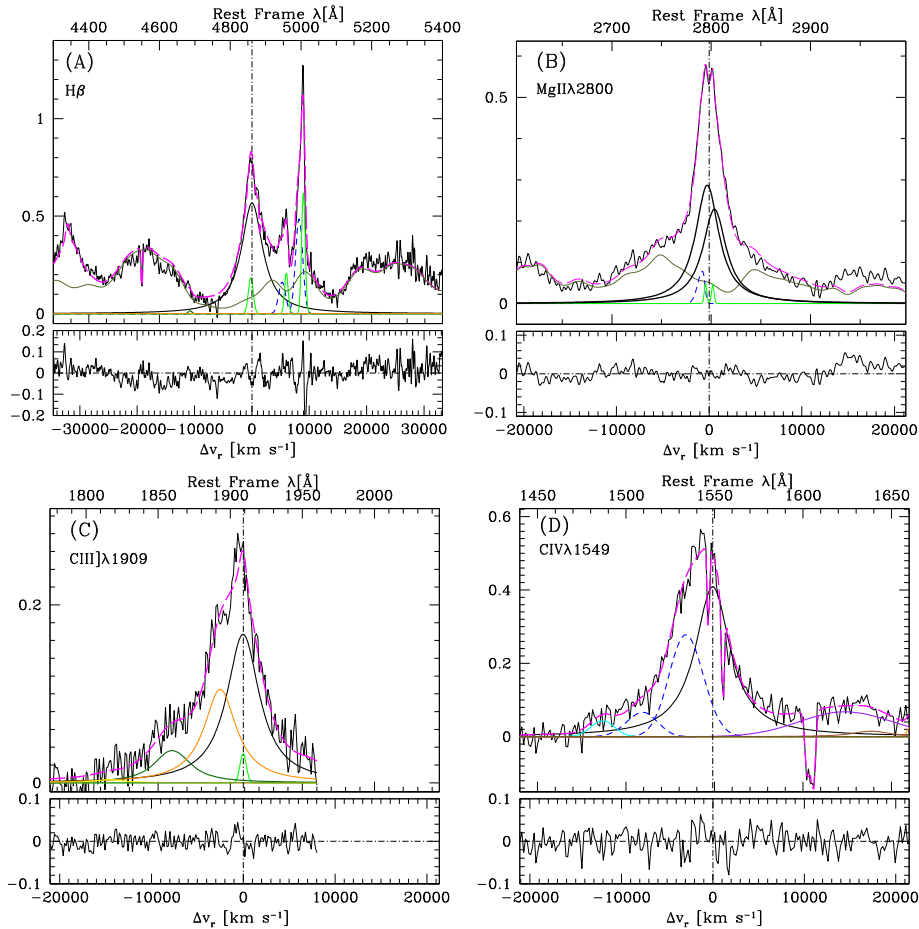
Figure 5. Multicomponent fits for 3C 57. H \beta and Mg II \lambda 2800 from CAHA spectrum and C III] \lambda 1909 and C IV \lambda 1549 from HST spectrum. The upper abscissa is rest-frame wavelength in \text{\AA} , the lower abscissa is in radial velocity units and the ordinate is specific flux per unit wavelength in arbitrary units. The vertical long dashed line indicates the adopted rest frame. The black lines show the original continuum-subtracted spectra while the dashed magenta indicates the fit to the entire spectrum. The thick black and thin green lines show the broad and narrow components, respectively. The blue-shifted component is indicated by a dashed blue line when detected. The light grey lines trace Fe II UV and Fe II opt emission which is considered in all four fittings. In some of them (as H \beta and Mg II \lambda 2800), the contribution is very important but in others (as C III] \lambda 1909 and C IV \lambda 1549) it is negligible. In panel (C), apart of C III] \lambda 1909 we show Si III] \lambda 1892, Al III \lambda 1860 and Si II \lambda 1814 in orange, dark green and yellow, respectively. In panel (D), together with C IV \lambda 1549 we plot the N IV] \lambda 1486 component in cyan and the He II \lambda 1640 broad and blue component in brown and violet, respectively.
